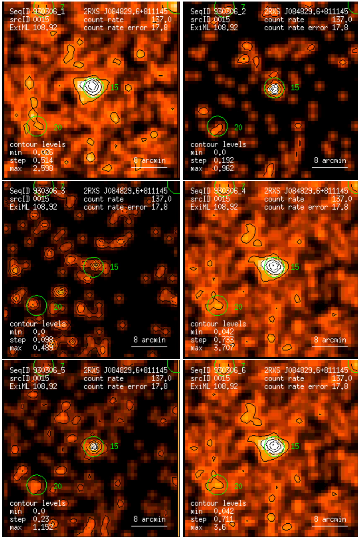
Figure 15: RASS 930306: detection 0015: band rate images, Gaussian filter: (1) PSPC channels 11 – 41, (2) 52 – 90, (3) 91 – 201, (4) 11 – 235, (5) 52 – 201, (6) 11 – 201. Broad band rates in counts/ks. Band rate contour levels in counts/ks/arcmin 2 .
