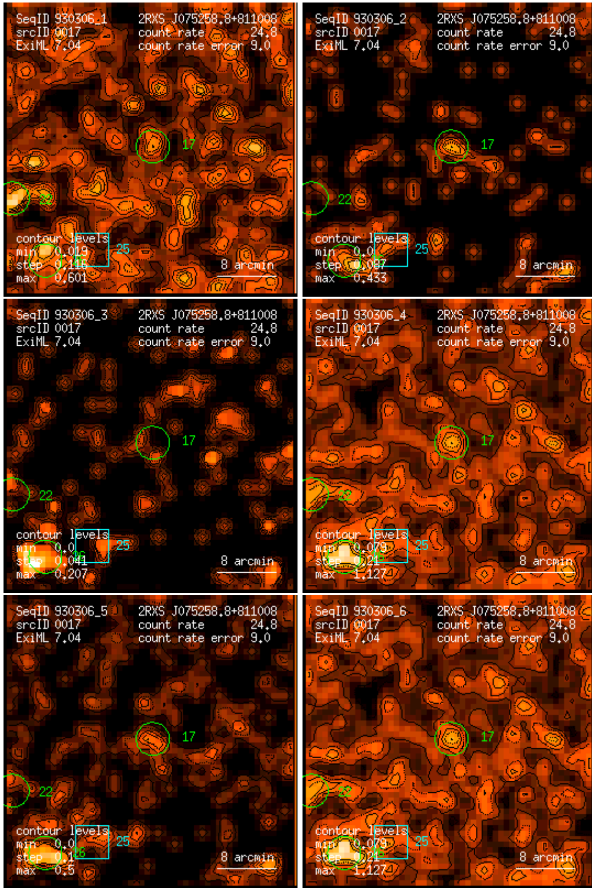
Figure 17: RASS 930306: detection 0017: band rate images, Gaussian filter: (1) PSPC channels 11 – 41, (2) 52 – 90, (3) 91 – 201, (4) 11 – 235, (5) 52 – 201, (6) 11 – 201. Broad band rates in counts/ks. Band rate contour levels in counts/ks/arcmin 2 .
