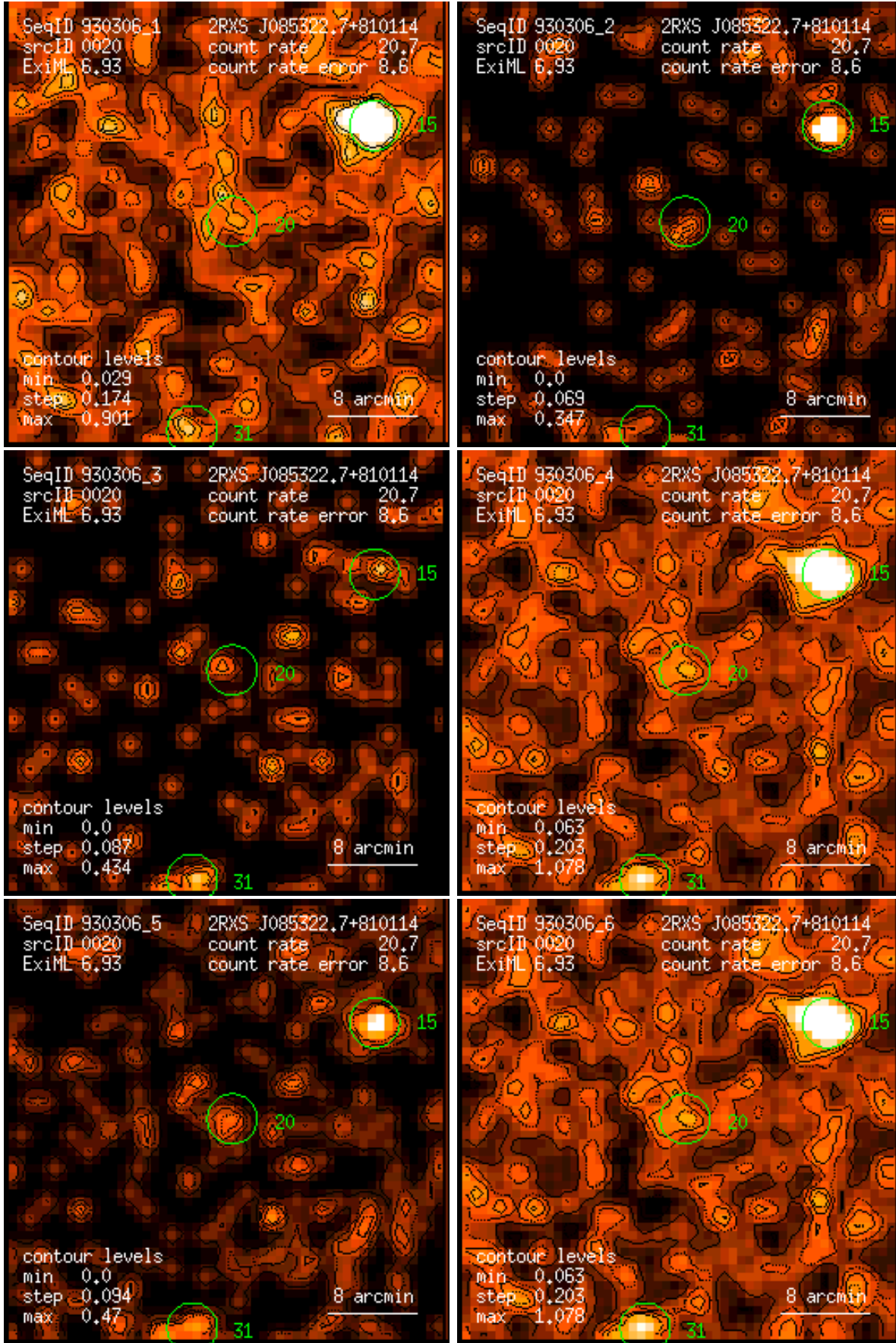
Figure 20: RASS 930306: detection 0020: band rate images, Gaussian filter: (1) PSPC channels 11 – 41, (2) 52 – 90, (3) 91 – 201, (4) 11 – 235, (5) 52 – 201, (6) 11 – 201. Broad band rates in counts/ks. Band rate contour levels in counts/ks/arcmin 2 .
