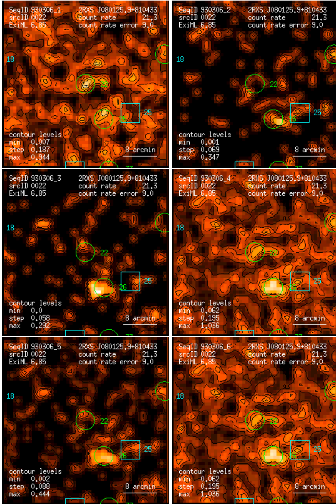
Figure 22: RASS 930306: detection 0022: band rate images, Gaussian filter: (1) PSPC channels 11 – 41, (2) 52 – 90, (3) 91 – 201, (4) 11 – 235, (5) 52 – 201, (6) 11 – 201. Broad band rates in counts/ks. Band rate contour levels in counts/ks/arcmin 2 .
