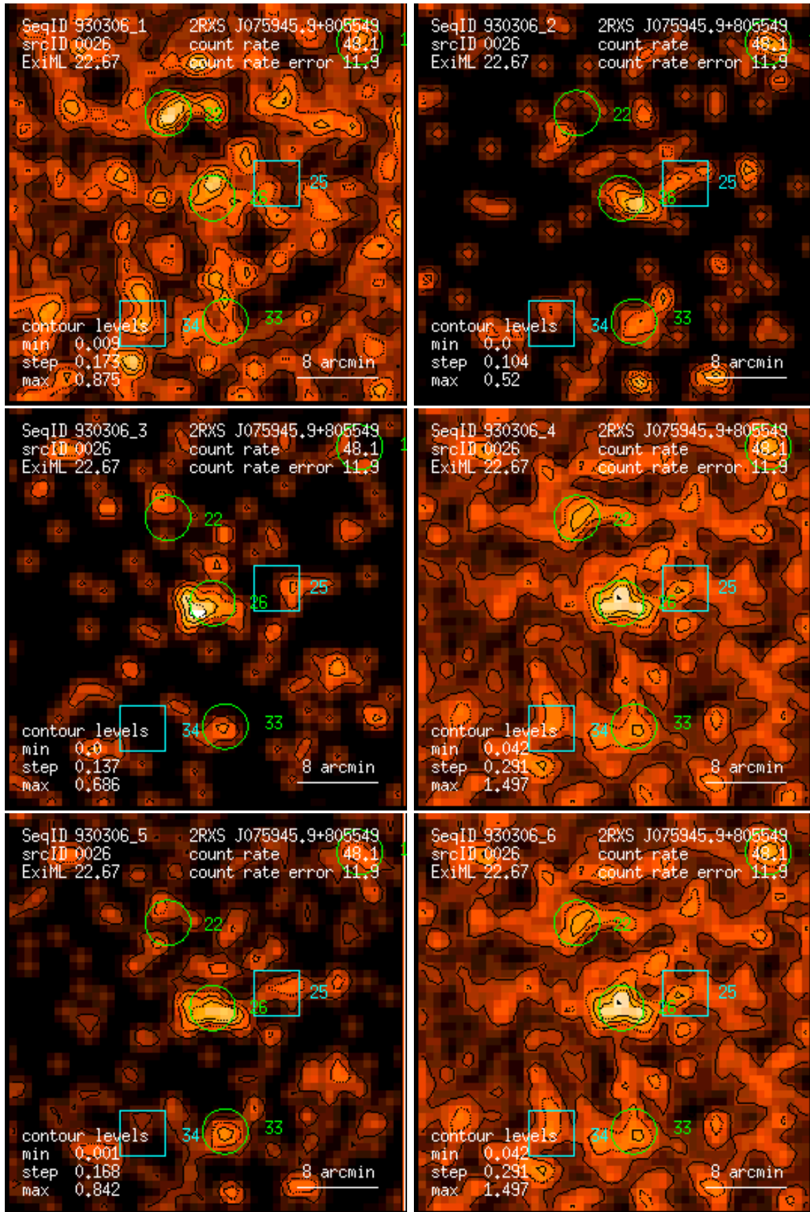
Figure 26: RASS 930306: detection 0026: band rate images, Gaussian filter: (1) PSPC channels 11 – 41, (2) 52 – 90, (3) 91 – 201, (4) 11 – 235, (5) 52 – 201, (6) 11 – 201. Broad band rates in counts/ks. Band rate contour levels in counts/ks/arcmin 2 .
