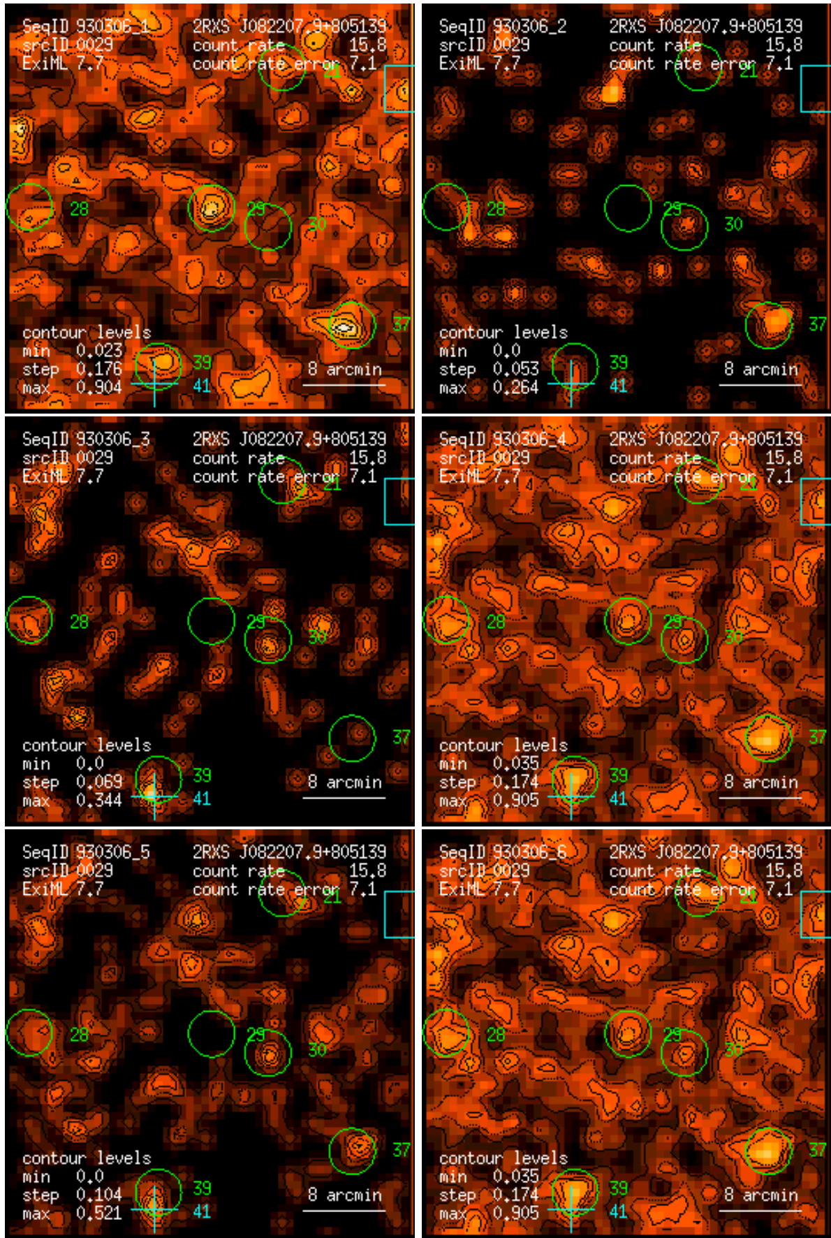
Figure 29: RASS 930306: detection 0029: band rate images, Gaussian filter: (1) PSPC channels 11 – 41, (2) 52 – 90, (3) 91 – 201, (4) 11 – 235, (5) 52 – 201, (6) 11 – 201. Broad band rates in counts/ks. Band rate contour levels in counts/ks/arcmin 2 .
