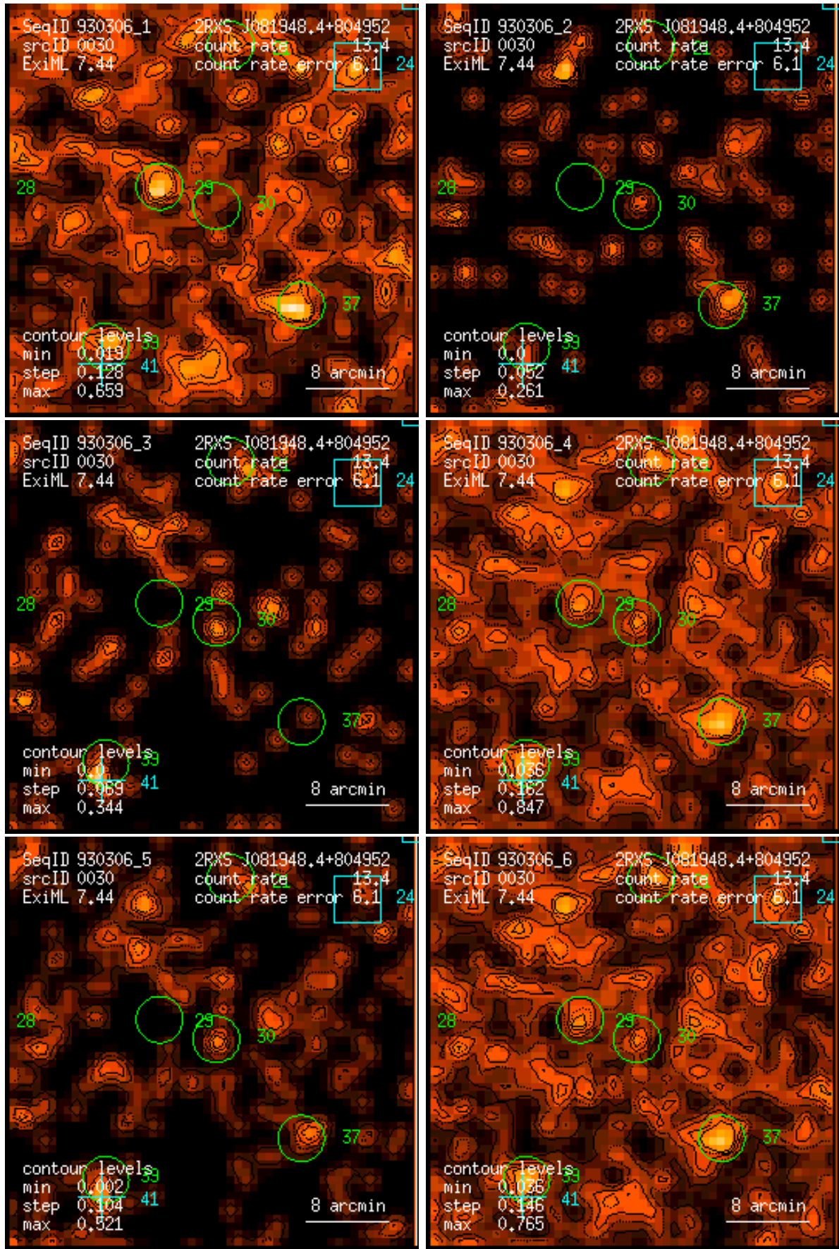
Figure 30: RASS 930306: detection 0030: band rate images, Gaussian filter: (1) PSPC channels 11 – 41, (2) 52 – 90, (3) 91 – 201, (4) 11 – 235, (5) 52 – 201, (6) 11 – 201. Broad band rates in counts/ks. Band rate contour levels in counts/ks/arcmin 2 .
