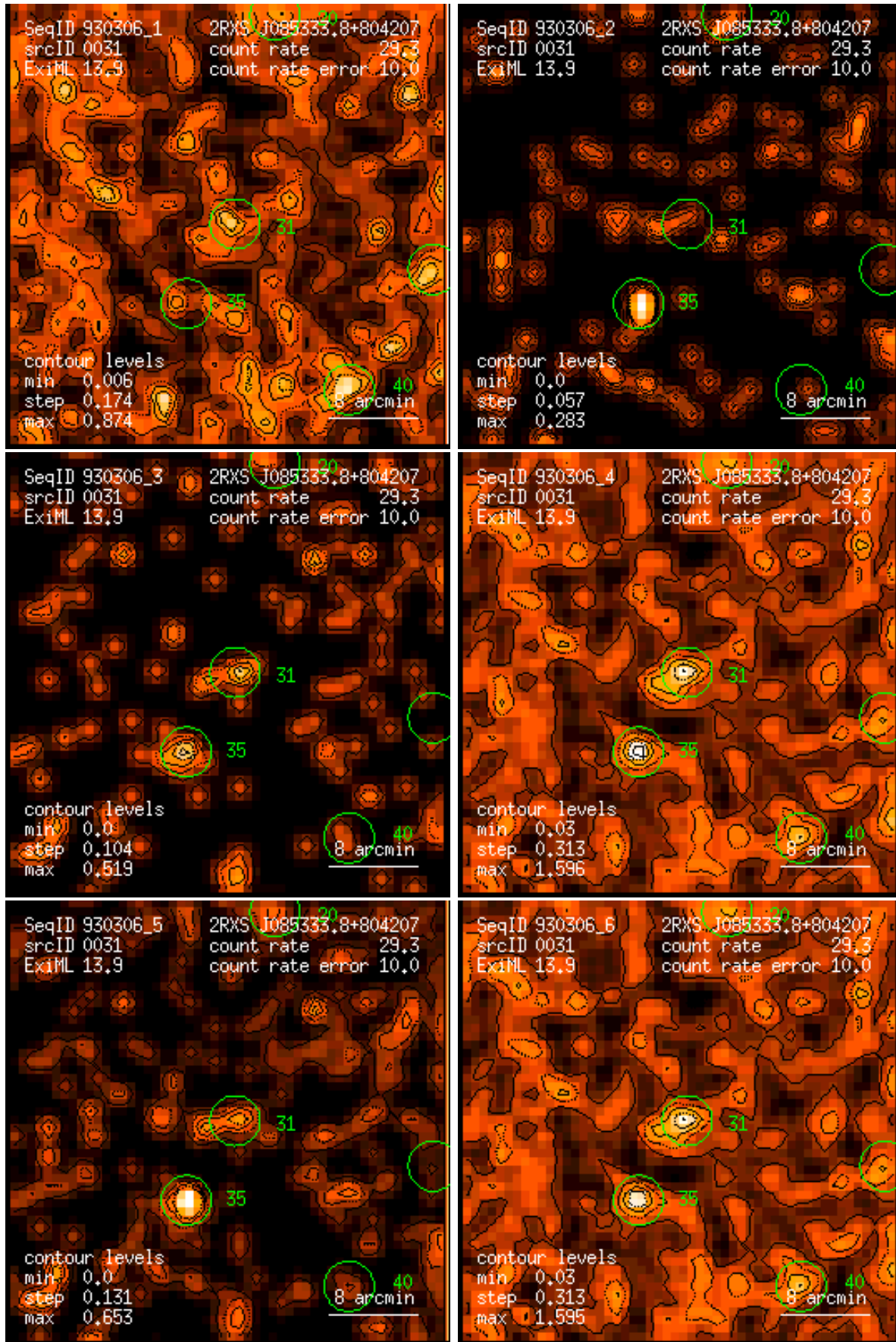
Figure 31: RASS 930306: detection 0031: band rate images, Gaussian filter: (1) PSPC channels 11 – 41, (2) 52 – 90, (3) 91 – 201, (4) 11 – 235, (5) 52 – 201, (6) 11 – 201. Broad band rates in counts/ks. Band rate contour levels in counts/ks/arcmin 2 .
