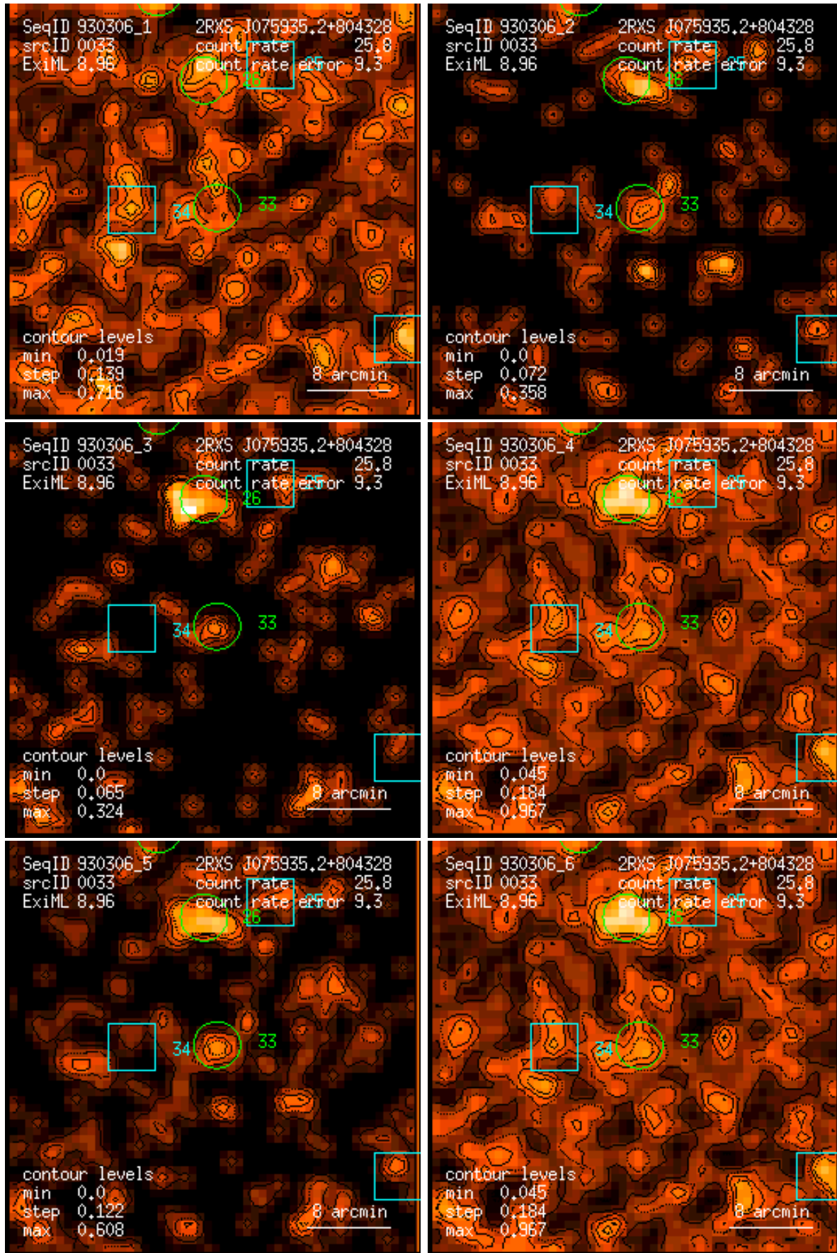
Figure 33: RASS 930306: detection 0033: band rate images, Gaussian filter: (1) PSPC channels 11 – 41, (2) 52 – 90, (3) 91 – 201, (4) 11 – 235, (5) 52 – 201, (6) 11 – 201. Broad band rates in counts/ks. Band rate contour levels in counts/ks/arcmin 2 .
