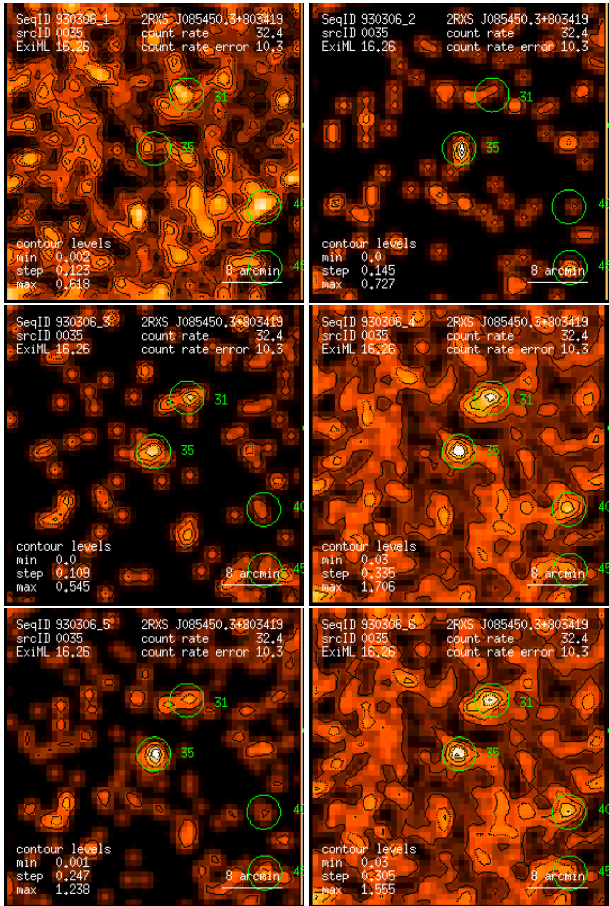
Figure 35: RASS 930306: detection 0035: band rate images, Gaussian filter: (1) PSPC channels 11 – 41, (2) 52 – 90, (3) 91 – 201, (4) 11 – 235, (5) 52 – 201, (6) 11 – 201. Broad band rates in counts/ks. Band rate contour levels in counts/ks/arcmin 2 .
