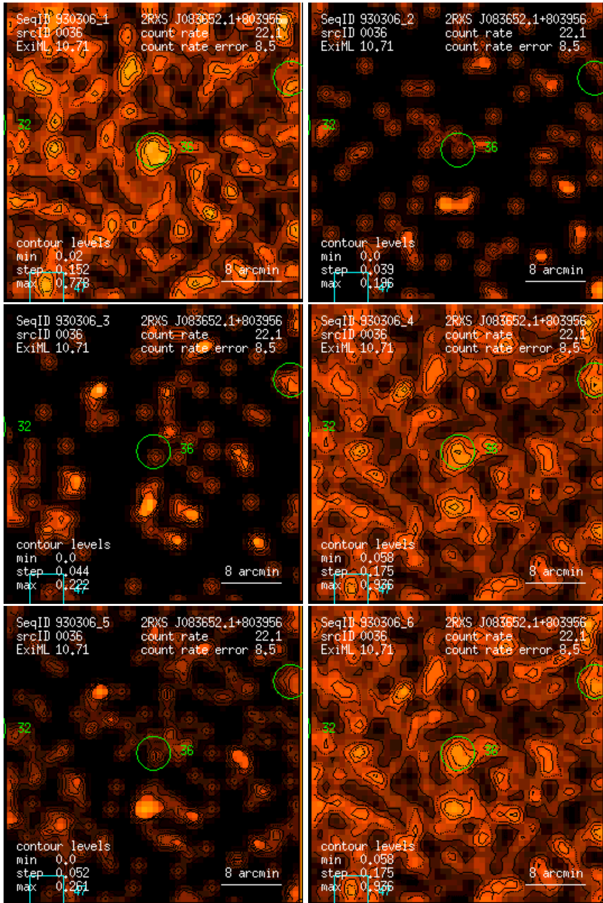
Figure 36: RASS 930306: detection 0036: band rate images, Gaussian filter: (1) PSPC channels 11 – 41, (2) 52 – 90, (3) 91 – 201, (4) 11 – 235, (5) 52 – 201, (6) 11 – 201. Broad band rates in counts/ks. Band rate contour levels in counts/ks/arcmin 2 .
