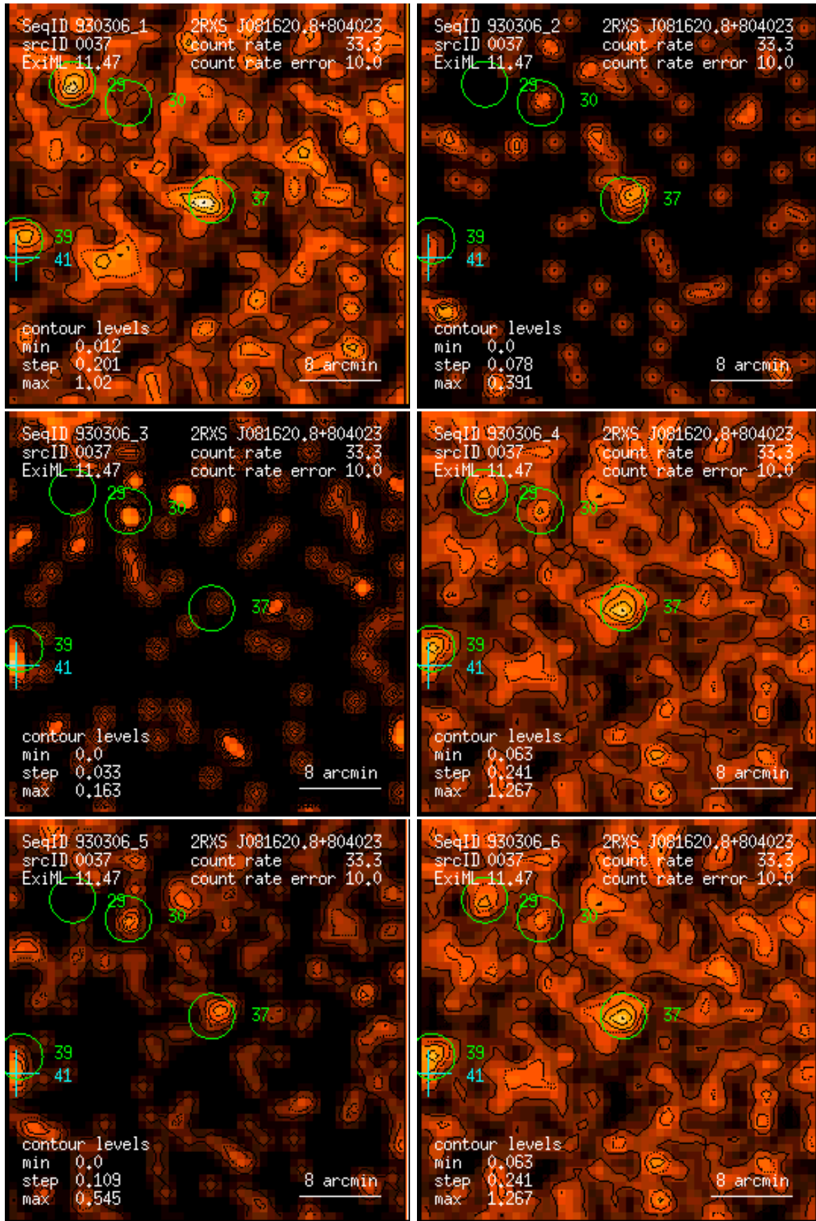
Figure 37: RASS 930306: detection 0037: band rate images, Gaussian filter: (1) PSPC channels 11 – 41, (2) 52 – 90, (3) 91 – 201, (4) 11 – 235, (5) 52 – 201, (6) 11 – 201. Broad band rates in counts/ks. Band rate contour levels in counts/ks/arcmin 2 .
