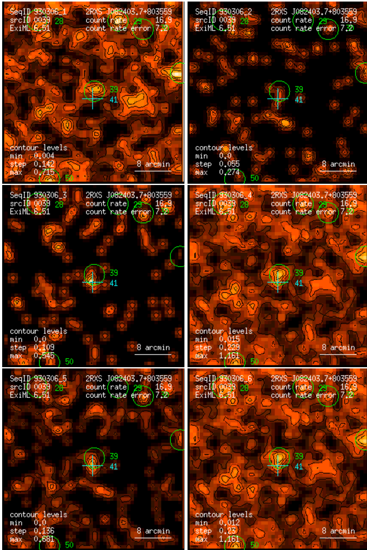
Figure 39: RASS 930306: detection 0039: band rate images, Gaussian filter: (1) PSPC channels 11 – 41, (2) 52 – 90, (3) 91 – 201, (4) 11 – 235, (5) 52 – 201, (6) 11 – 201. Broad band rates in counts/ks. Band rate contour levels in counts/ks/arcmin 2 .
