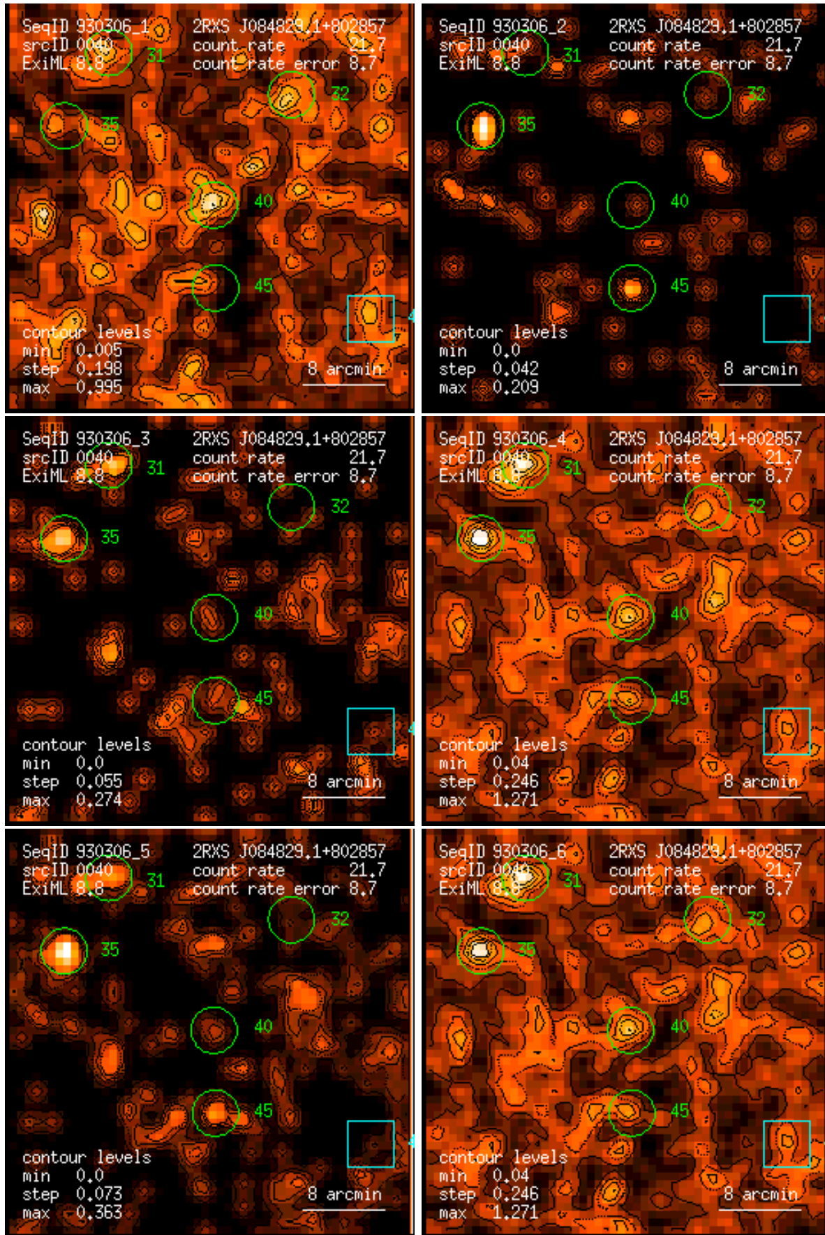
Figure 40: RASS 930306: detection 0040: band rate images, Gaussian filter: (1) PSPC channels 11 – 41, (2) 52 – 90, (3) 91 – 201, (4) 11 – 235, (5) 52 – 201, (6) 11 – 201. Broad band rates in counts/ks. Band rate contour levels in counts/ks/arcmin 2 .
