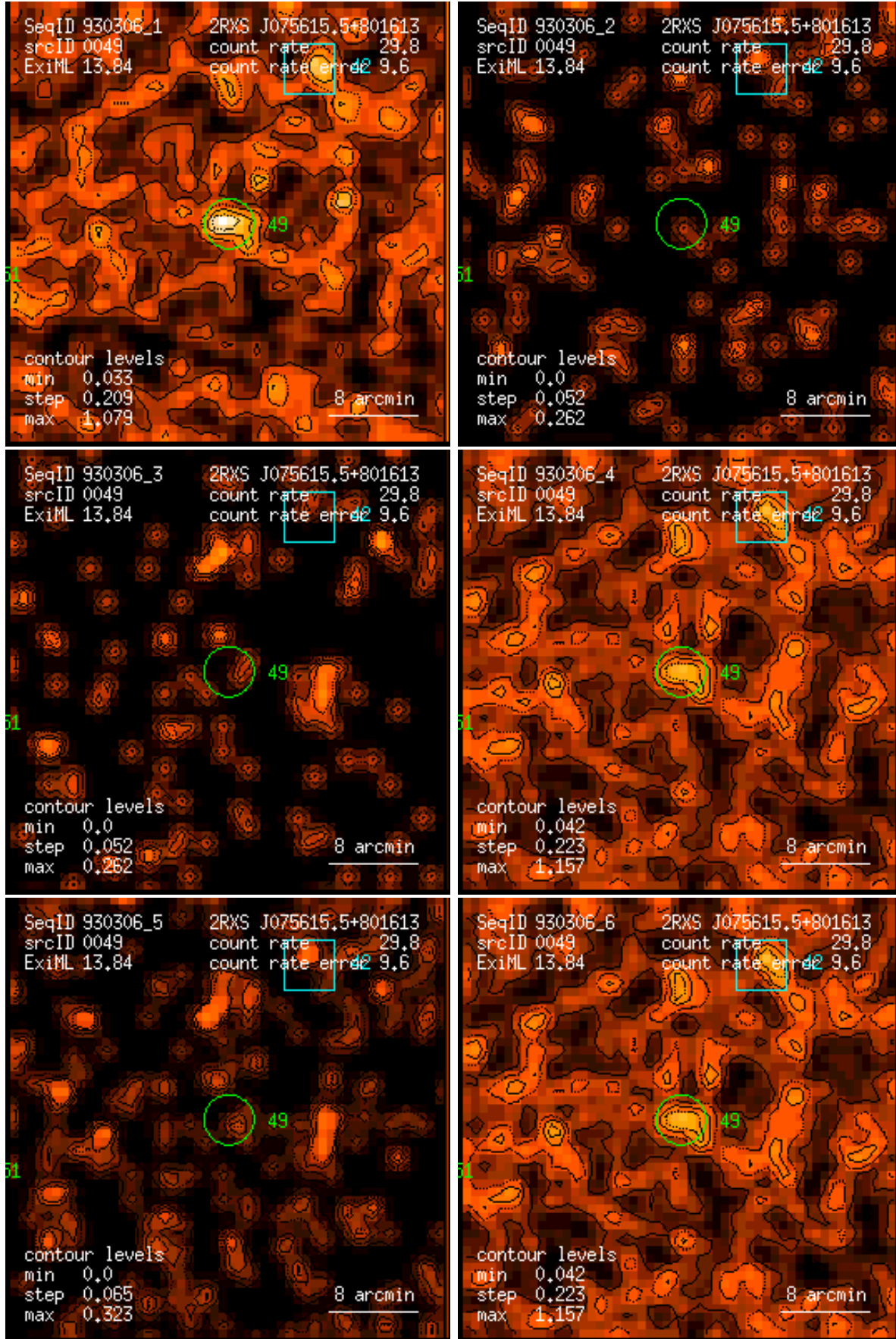
Figure 49: RASS 930306: detection 0049: band rate images, Gaussian filter: (1) PSPC channels 11 – 41, (2) 52 – 90, (3) 91 – 201, (4) 11 – 235, (5) 52 – 201, (6) 11 – 201. Broad band rates in counts/ks. Band rate contour levels in counts/ks/arcmin 2 .
