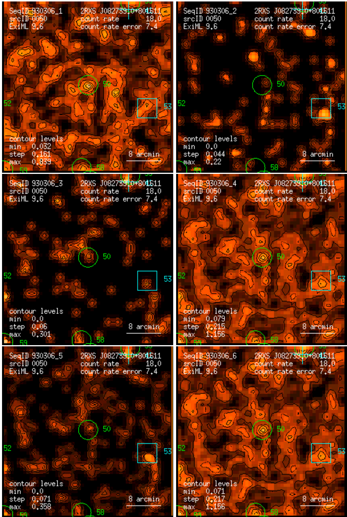
Figure 50: RASS 930306: detection 0050: band rate images, Gaussian filter: (1) PSPC channels 11 – 41, (2) 52 – 90, (3) 91 – 201, (4) 11 – 235, (5) 52 – 201, (6) 11 – 201. Broad band rates in counts/ks. Band rate contour levels in counts/ks/arcmin 2 .
