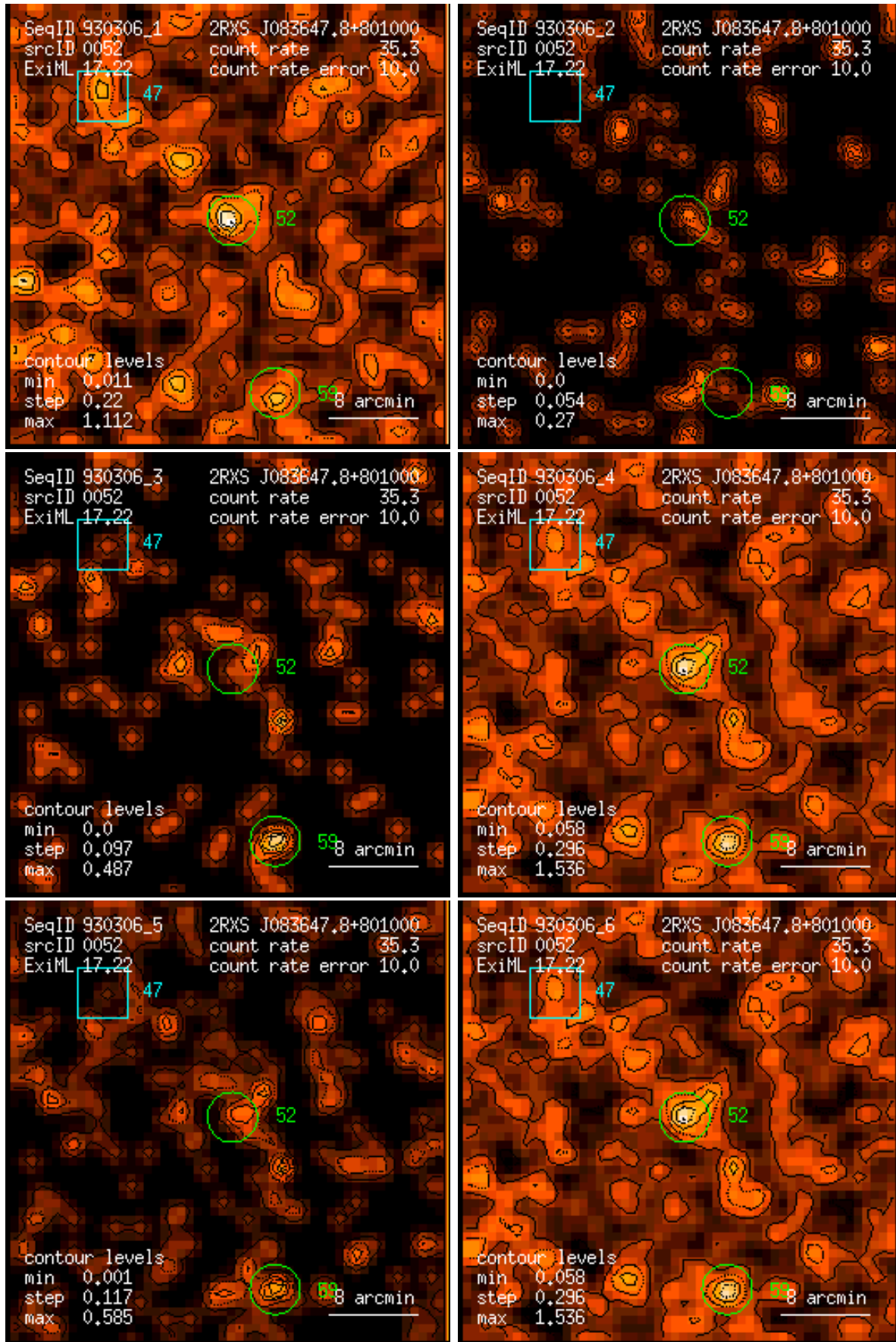
Figure 52: RASS 930306: detection 0052: band rate images, Gaussian filter: (1) PSPC channels 11 – 41, (2) 52 – 90, (3) 91 – 201, (4) 11 – 235, (5) 52 – 201, (6) 11 – 201. Broad band rates in counts/ks. Band rate contour levels in counts/ks/arcmin 2 .
