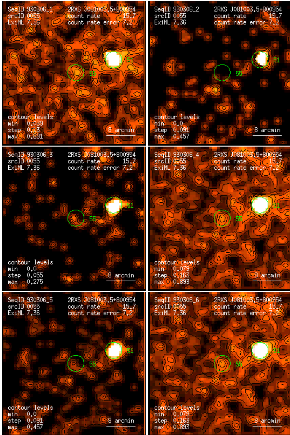
Figure 55: RASS 930306: detection 0055: band rate images, Gaussian filter: (1) PSPC channels 11 – 41, (2) 52 – 90, (3) 91 – 201, (4) 11 – 235, (5) 52 – 201, (6) 11 – 201. Broad band rates in counts/ks. Band rate contour levels in counts/ks/arcmin 2 .
