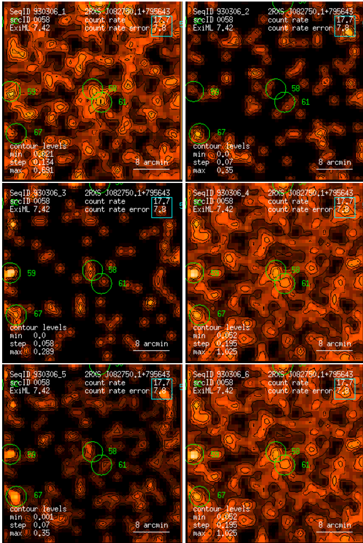
Figure 58: RASS 930306: detection 0058: band rate images, Gaussian filter: (1) PSPC channels 11 – 41, (2) 52 – 90, (3) 91 – 201, (4) 11 – 235, (5) 52 – 201, (6) 11 – 201. Broad band rates in counts/ks. Band rate contour levels in counts/ks/arcmin 2 .
