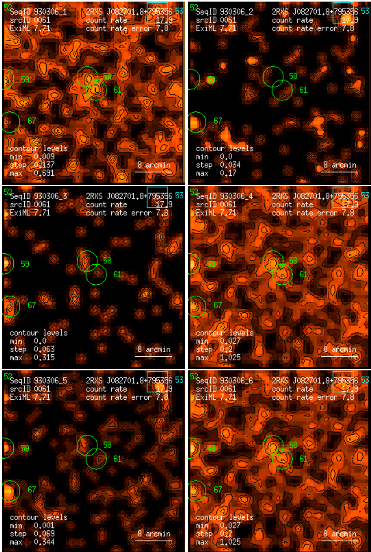
Figure 61: RASS 930306: detection 0061: band rate images, Gaussian filter: (1) PSPC channels 11 – 41, (2) 52 – 90, (3) 91 – 201, (4) 11 – 235, (5) 52 – 201, (6) 11 – 201. Broad band rates in counts/ks. Band rate contour levels in counts/ks/arcmin 2 .
