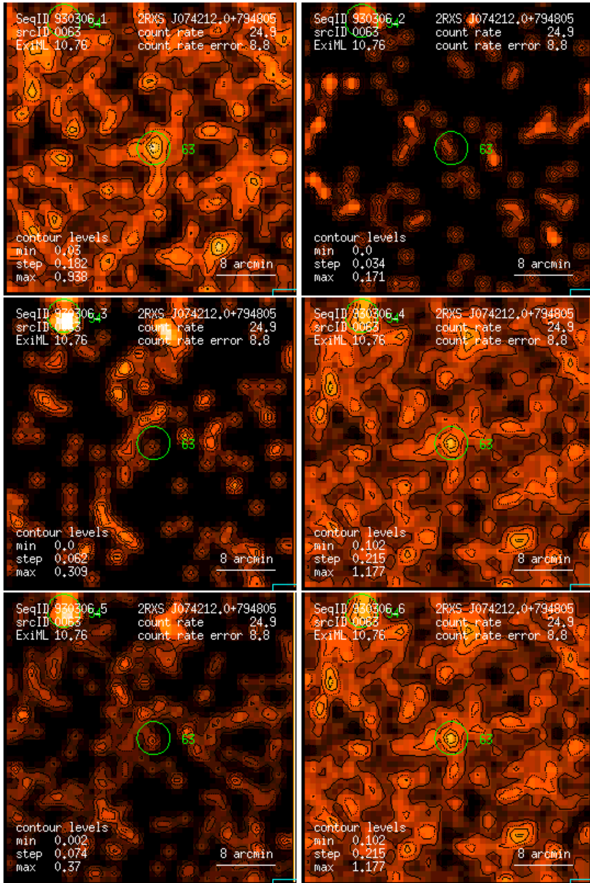
Figure 63: RASS 930306: detection 0063: band rate images, Gaussian filter: (1) PSPC channels 11 – 41, (2) 52 – 90, (3) 91 – 201, (4) 11 – 235, (5) 52 – 201, (6) 11 – 201. Broad band rates in counts/ks. Band rate contour levels in counts/ks/arcmin 2 .
