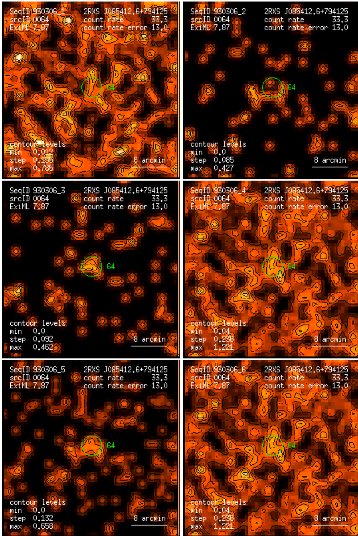
Figure 64: RASS 930306: detection 0064: band rate images, Gaussian filter: (1) PSPC channels 11 – 41, (2) 52 – 90, (3) 91 – 201, (4) 11 – 235, (5) 52 – 201, (6) 11 – 201. Broad band rates in counts/ks. Band rate contour levels in counts/ks/arcmin 2 .
