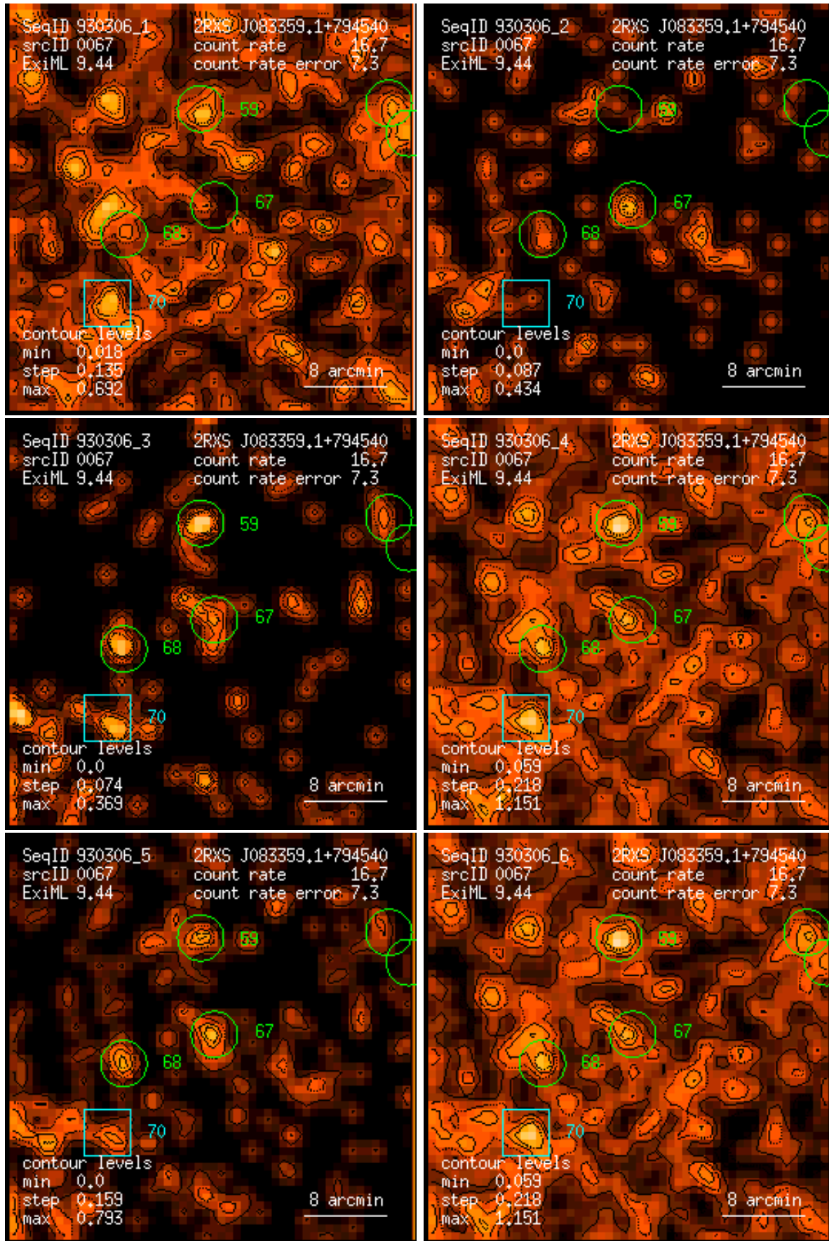
Figure 67: RASS 930306: detection 0067: band rate images, Gaussian filter: (1) PSPC channels 11 – 41, (2) 52 – 90, (3) 91 – 201, (4) 11 – 235, (5) 52 – 201, (6) 11 – 201. Broad band rates in counts/ks. Band rate contour levels in counts/ks/arcmin 2 .
