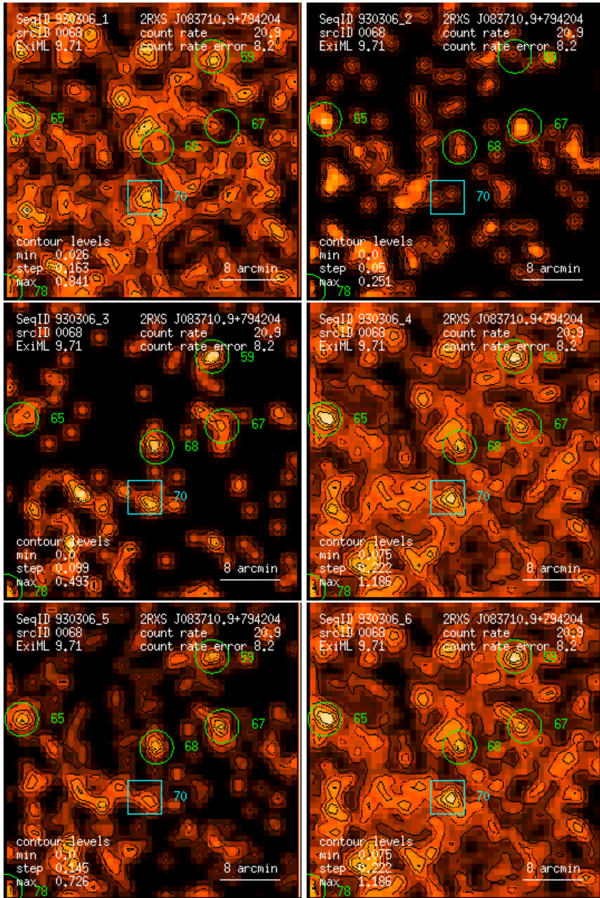
Figure 68: RASS 930306: detection 0068: band rate images, Gaussian filter: (1) PSPC channels 11 – 41, (2) 52 – 90, (3) 91 – 201, (4) 11 – 235, (5) 52 – 201, (6) 11 – 201. Broad band rates in counts/ks. Band rate contour levels in counts/ks/arcmin 2 .
