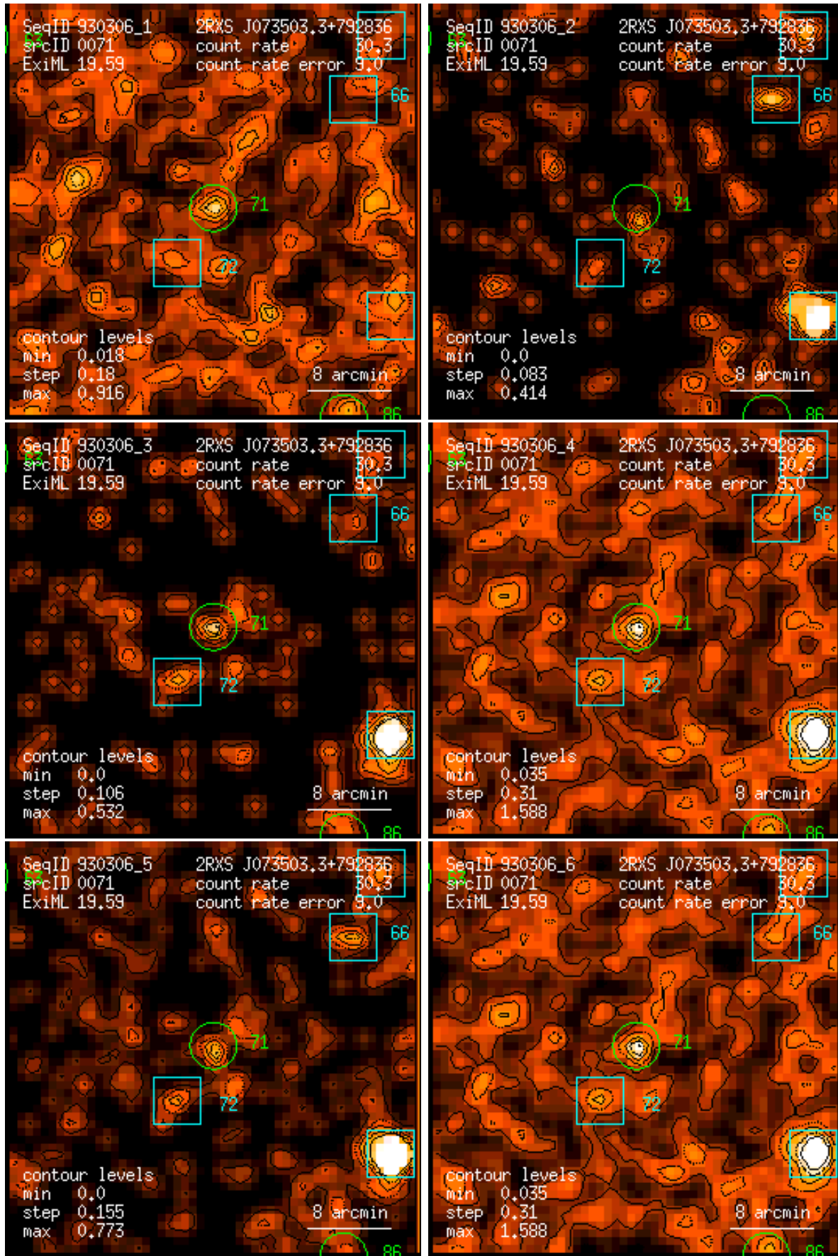
Figure 71: RASS 930306: detection 0071: band rate images, Gaussian filter: (1) PSPC channels 11 – 41, (2) 52 – 90, (3) 91 – 201, (4) 11 – 235, (5) 52 – 201, (6) 11 – 201. Broad band rates in counts/ks. Band rate contour levels in counts/ks/arcmin 2 .
