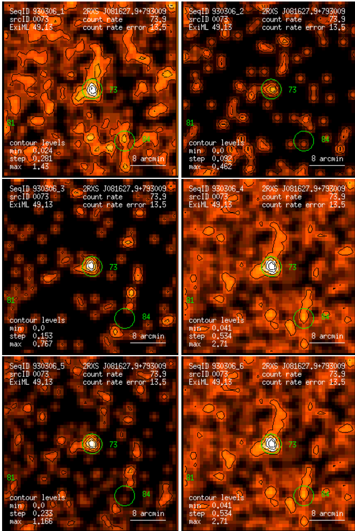
Figure 73: RASS 930306: detection 0073: band rate images, Gaussian filter: (1) PSPC channels 11 – 41, (2) 52 – 90, (3) 91 – 201, (4) 11 – 235, (5) 52 – 201, (6) 11 – 201. Broad band rates in counts/ks. Band rate contour levels in counts/ks/arcmin 2 .
