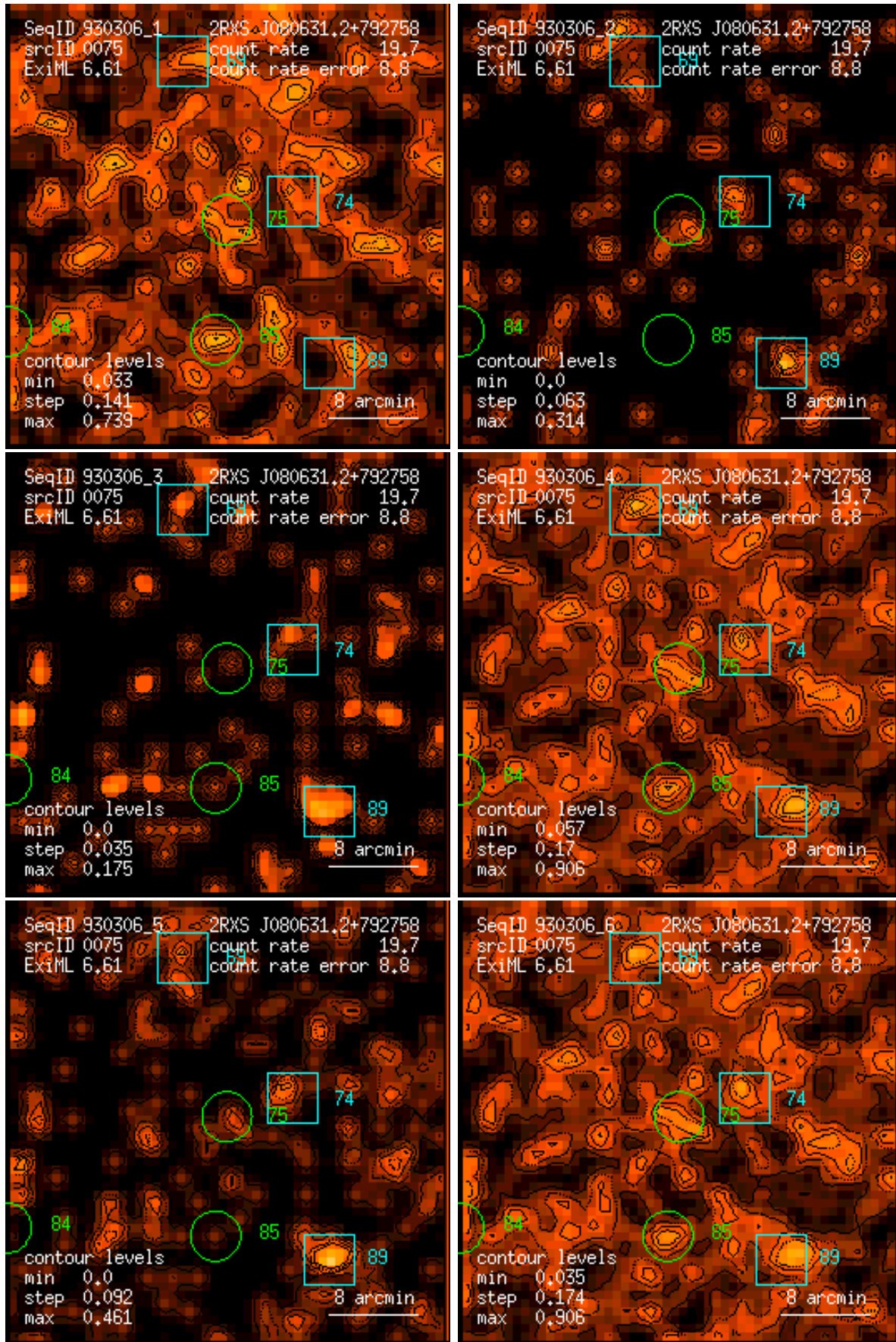
Figure 75: RASS 930306: detection 0075: band rate images, Gaussian filter: (1) PSPC channels 11 – 41, (2) 52 – 90, (3) 91 – 201, (4) 11 – 235, (5) 52 – 201, (6) 11 – 201. Broad band rates in counts/ks. Band rate contour levels in counts/ks/arcmin 2 .
