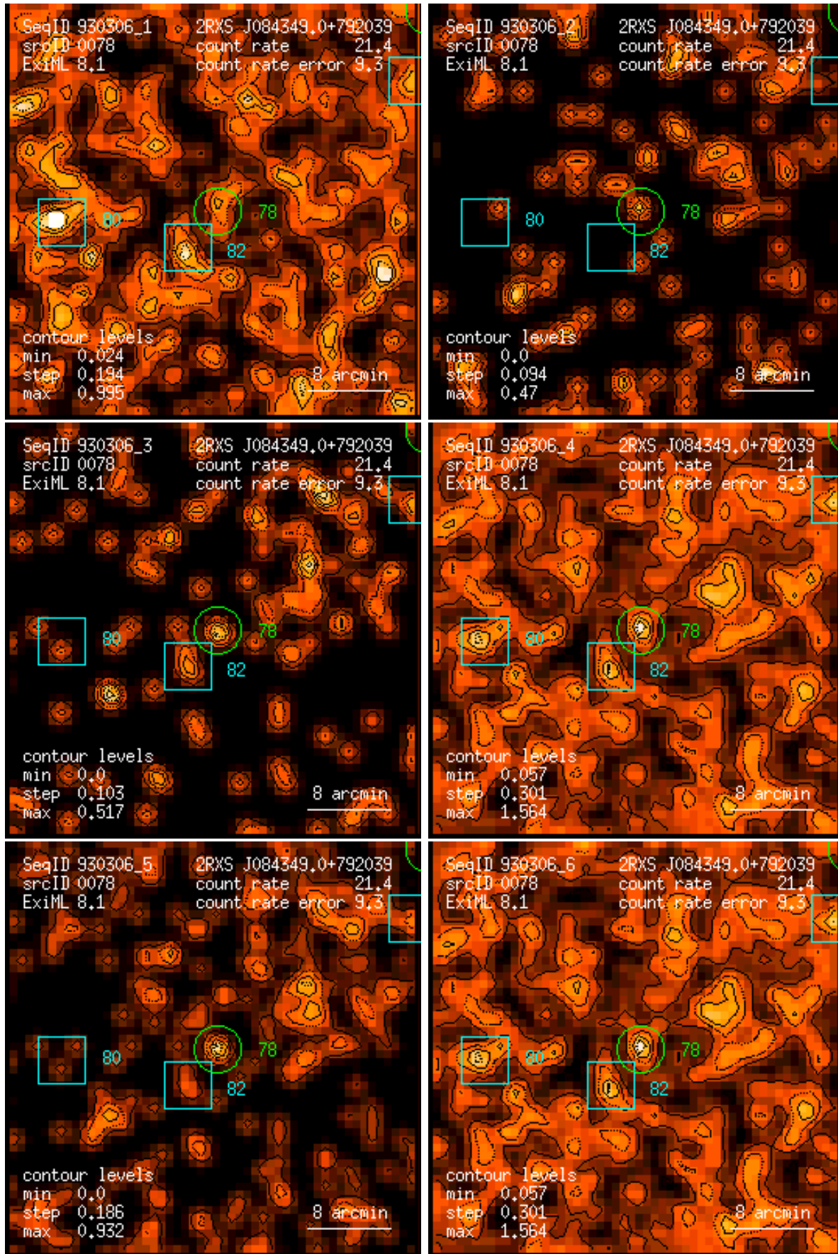
Figure 78: RASS 930306: detection 0078: band rate images, Gaussian filter: (1) PSPC channels 11 – 41, (2) 52 – 90, (3) 91 – 201, (4) 11 – 235, (5) 52 – 201, (6) 11 – 201. Broad band rates in counts/ks. Band rate contour levels in counts/ks/arcmin 2 .
