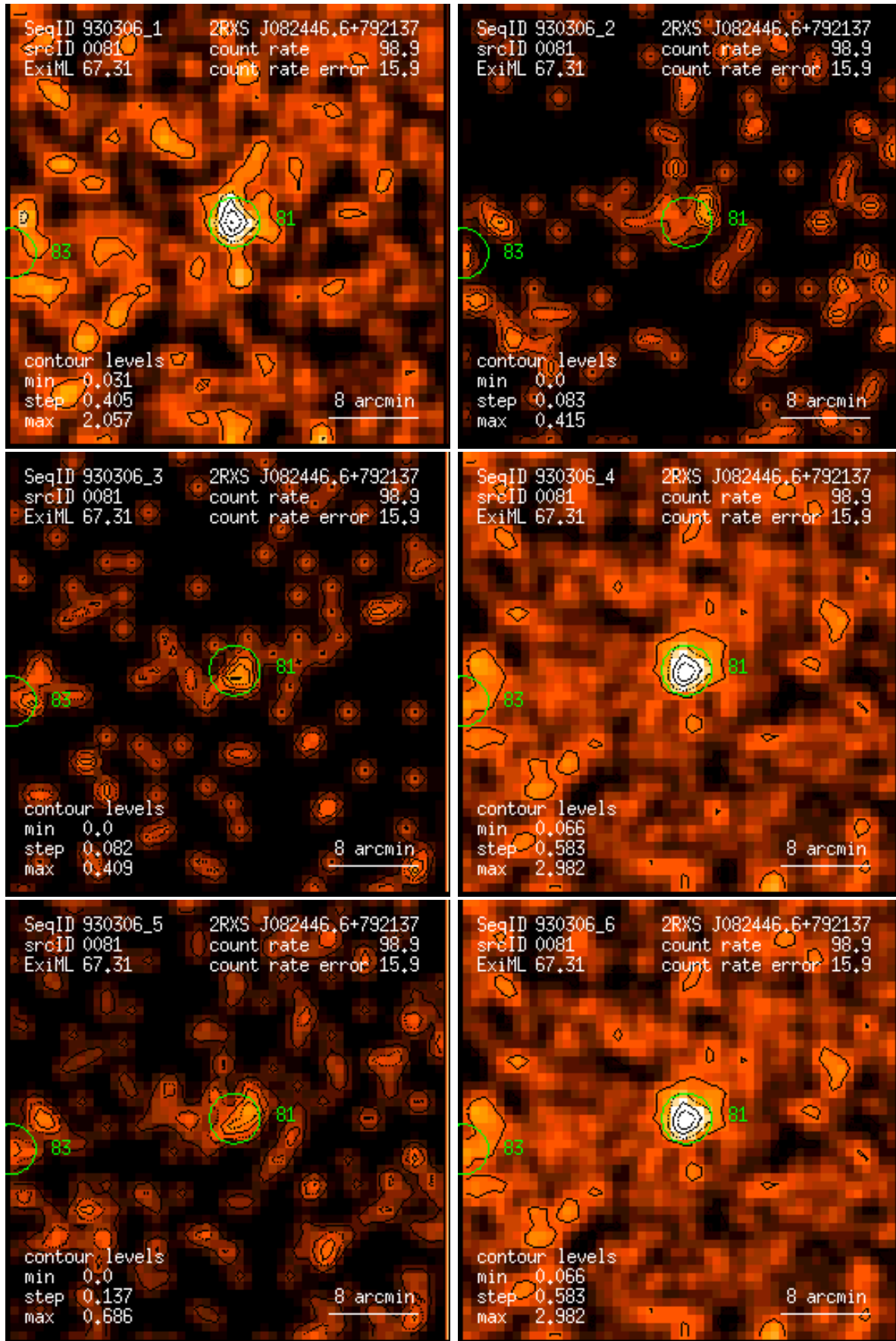
Figure 81: RASS 930306: detection 0081: band rate images, Gaussian filter: (1) PSPC channels 11 – 41, (2) 52 – 90, (3) 91 – 201, (4) 11 – 235, (5) 52 – 201, (6) 11 – 201. Broad band rates in counts/ks. Band rate contour levels in counts/ks/arcmin 2 .
