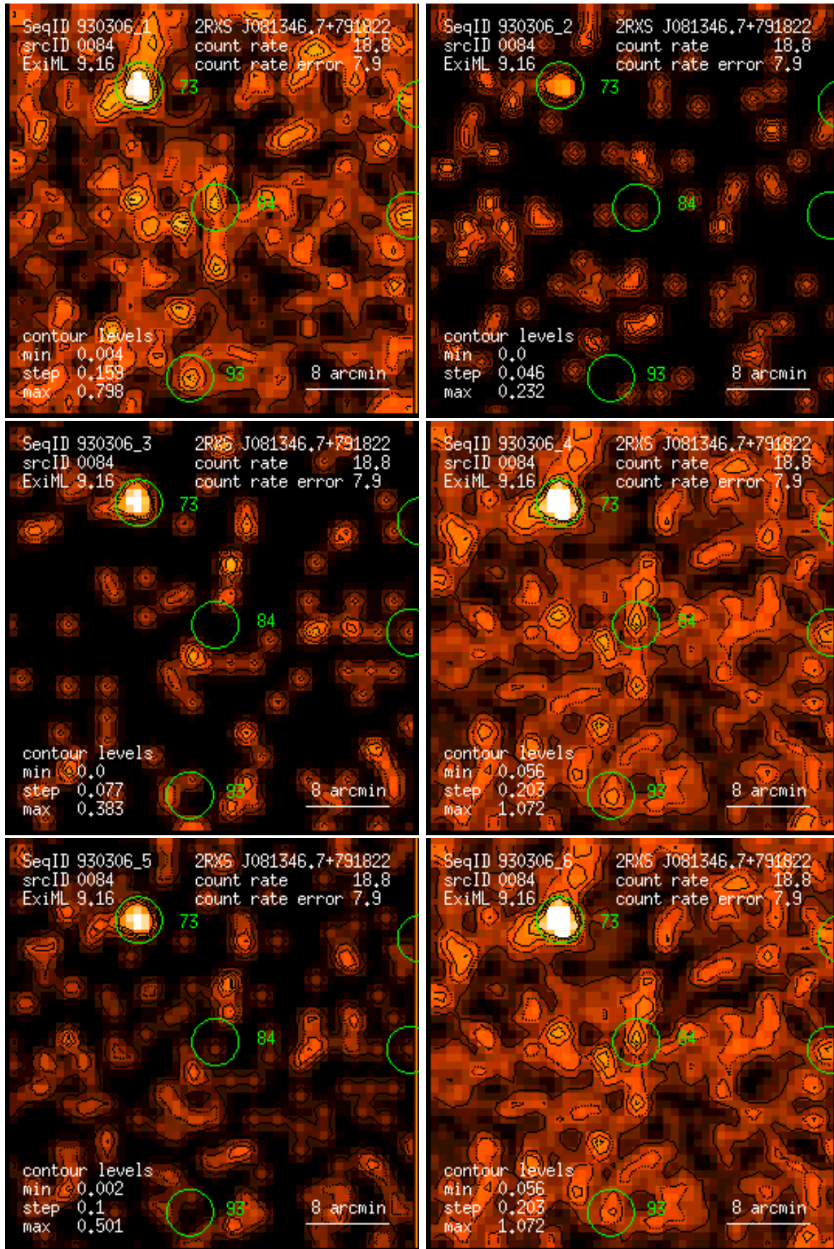
Figure 84: RASS 930306: detection 0084: band rate images, Gaussian filter: (1) PSPC channels 11 – 41, (2) 52 – 90, (3) 91 – 201, (4) 11 – 235, (5) 52 – 201, (6) 11 – 201. Broad band rates in counts/ks. Band rate contour levels in counts/ks/arcmin 2 .
