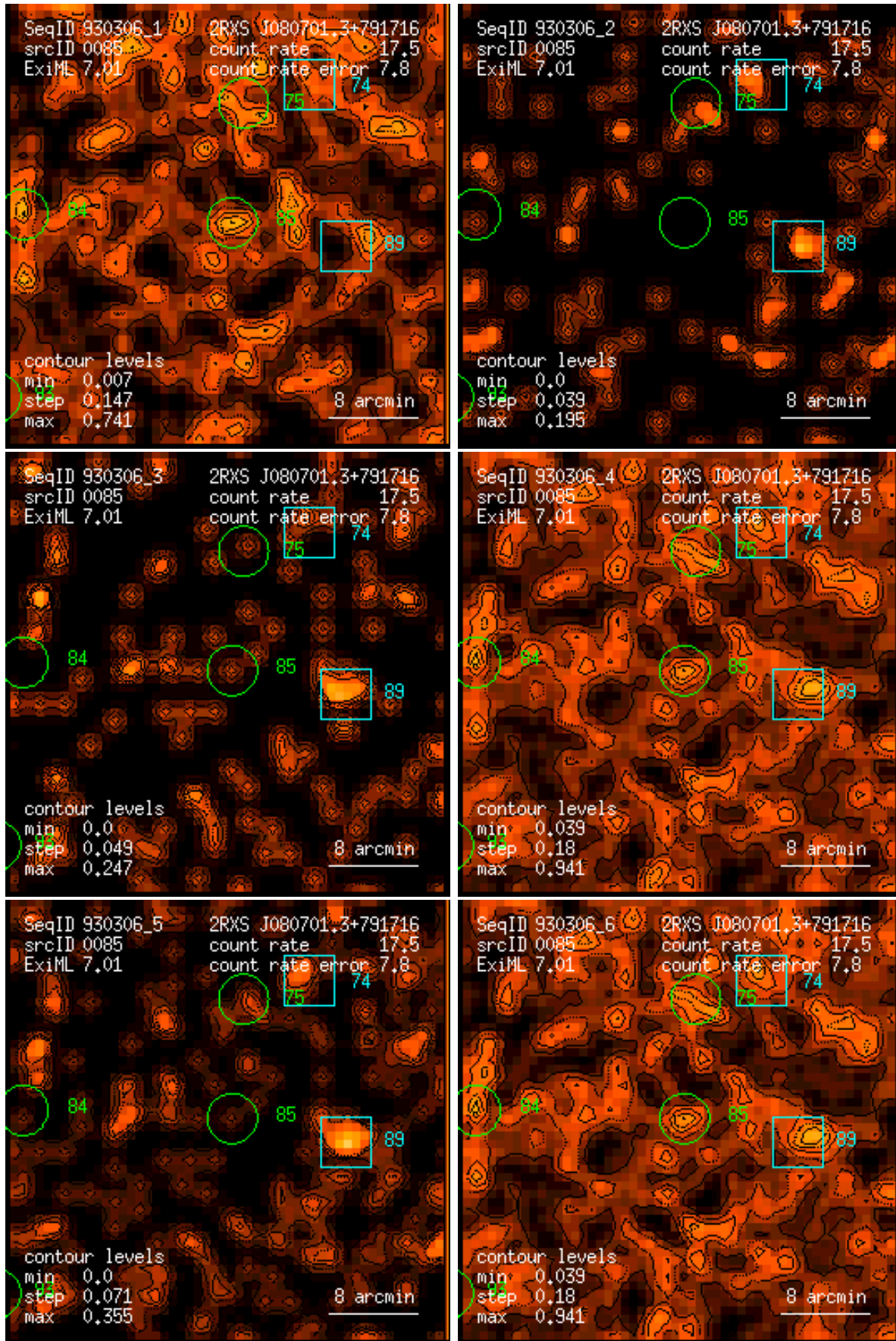
Figure 85: RASS 930306: detection 0085: band rate images, Gaussian filter: (1) PSPC channels 11 – 41, (2) 52 – 90, (3) 91 – 201, (4) 11 – 235, (5) 52 – 201, (6) 11 – 201. Broad band rates in counts/ks. Band rate contour levels in counts/ks/arcmin 2 .
