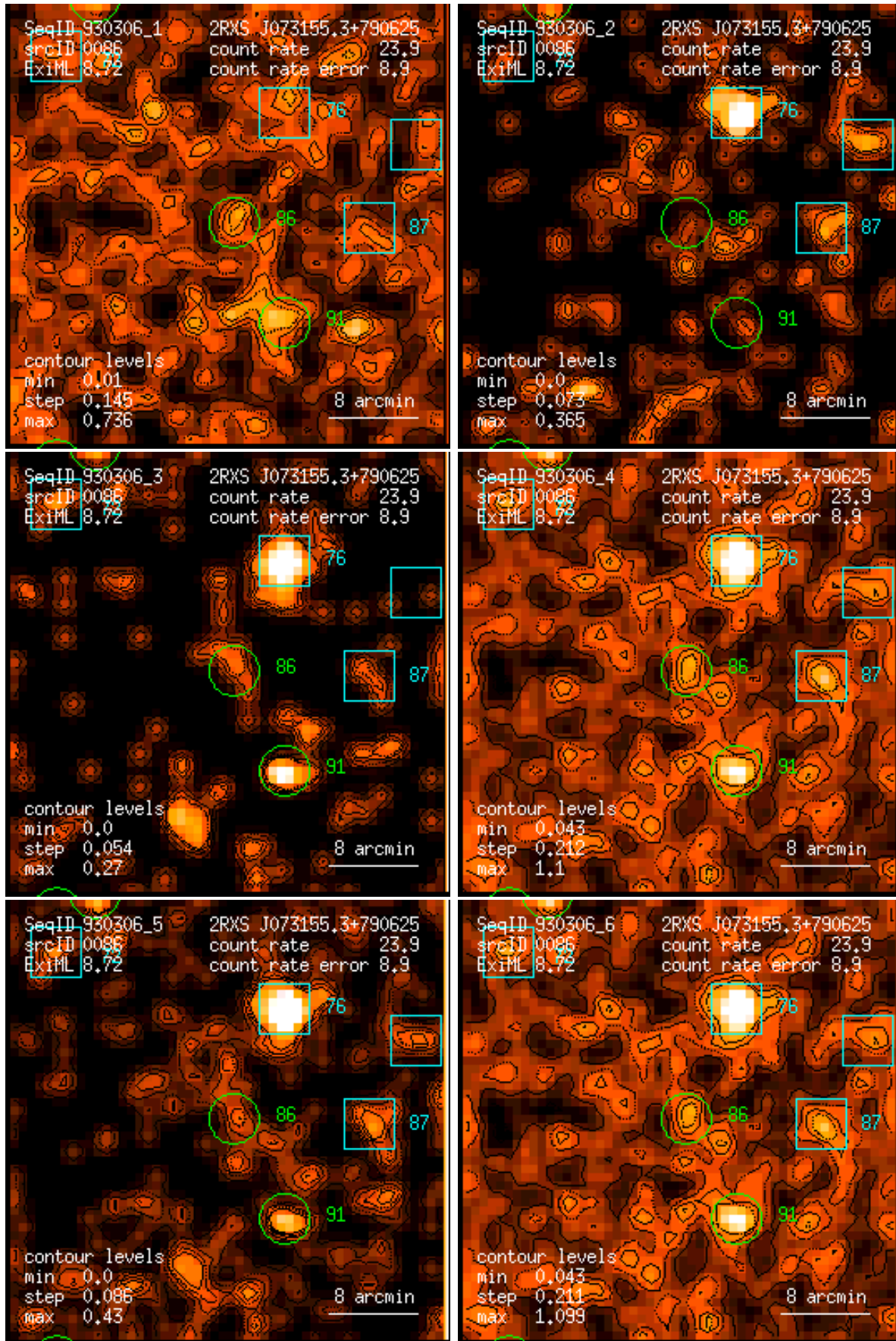
Figure 86: RASS 930306: detection 0086: band rate images, Gaussian filter: (1) PSPC channels 11 – 41, (2) 52 – 90, (3) 91 – 201, (4) 11 – 235, (5) 52 – 201, (6) 11 – 201. Broad band rates in counts/ks. Band rate contour levels in counts/ks/arcmin 2 .
