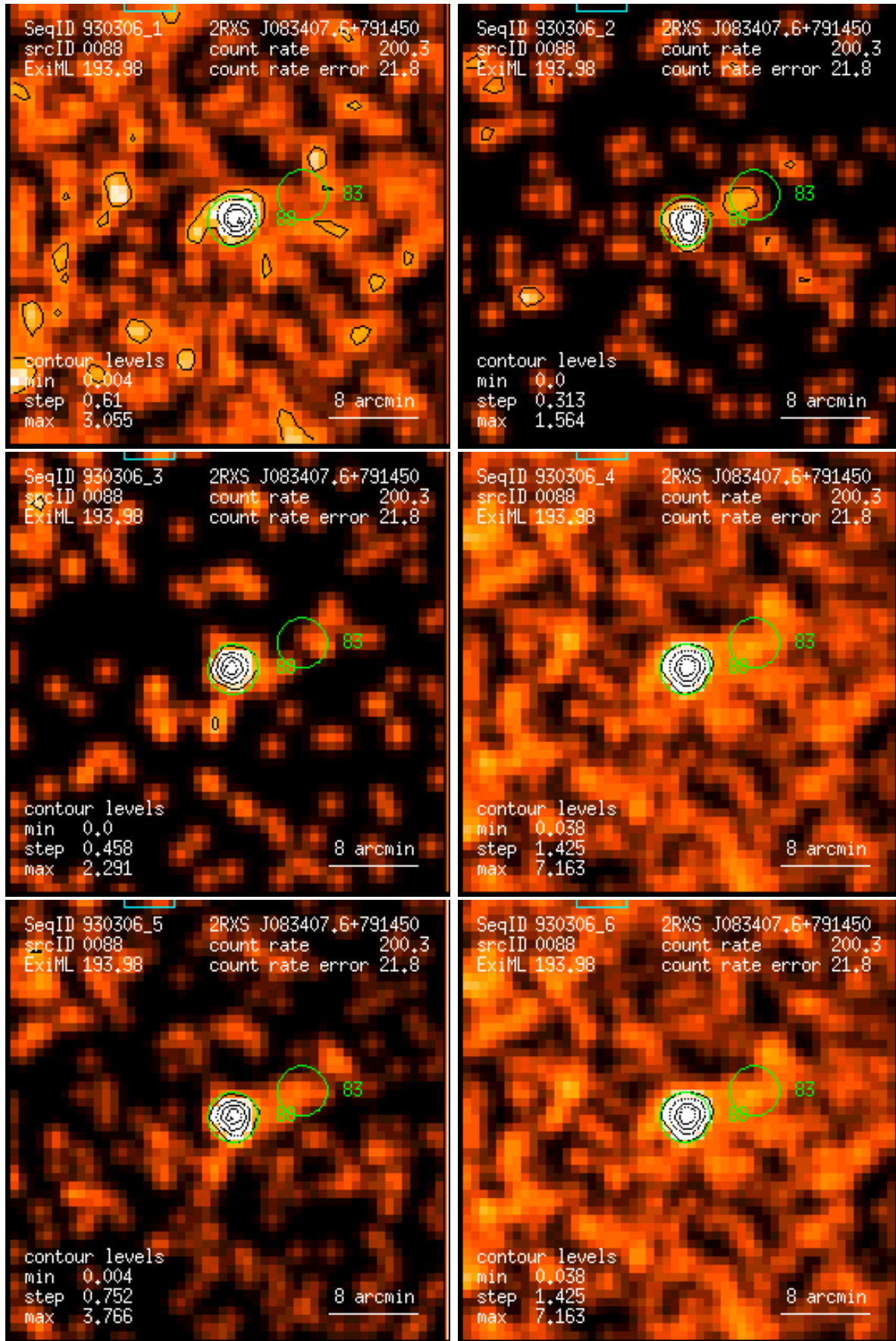
Figure 88: RASS 930306: detection 0088: band rate images, Gaussian filter: (1) PSPC channels 11 – 41, (2) 52 – 90, (3) 91 – 201, (4) 11 – 235, (5) 52 – 201, (6) 11 – 201. Broad band rates in counts/ks. Band rate contour levels in counts/ks/arcmin 2 .
