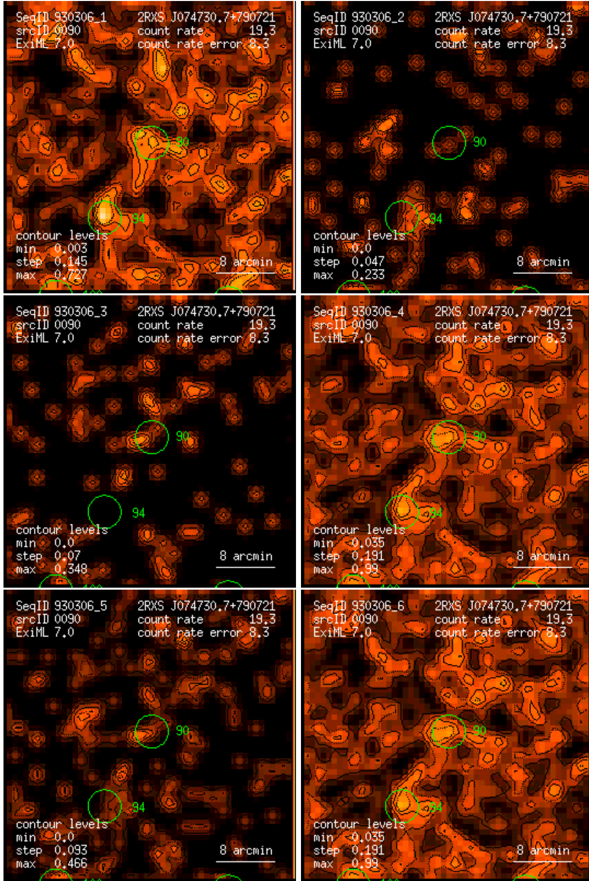
Figure 90: RASS 930306: detection 0090: band rate images, Gaussian filter: (1) PSPC channels 11 – 41, (2) 52 – 90, (3) 91 – 201, (4) 11 – 235, (5) 52 – 201, (6) 11 – 201. Broad band rates in counts/ks. Band rate contour levels in counts/ks/arcmin 2 .
