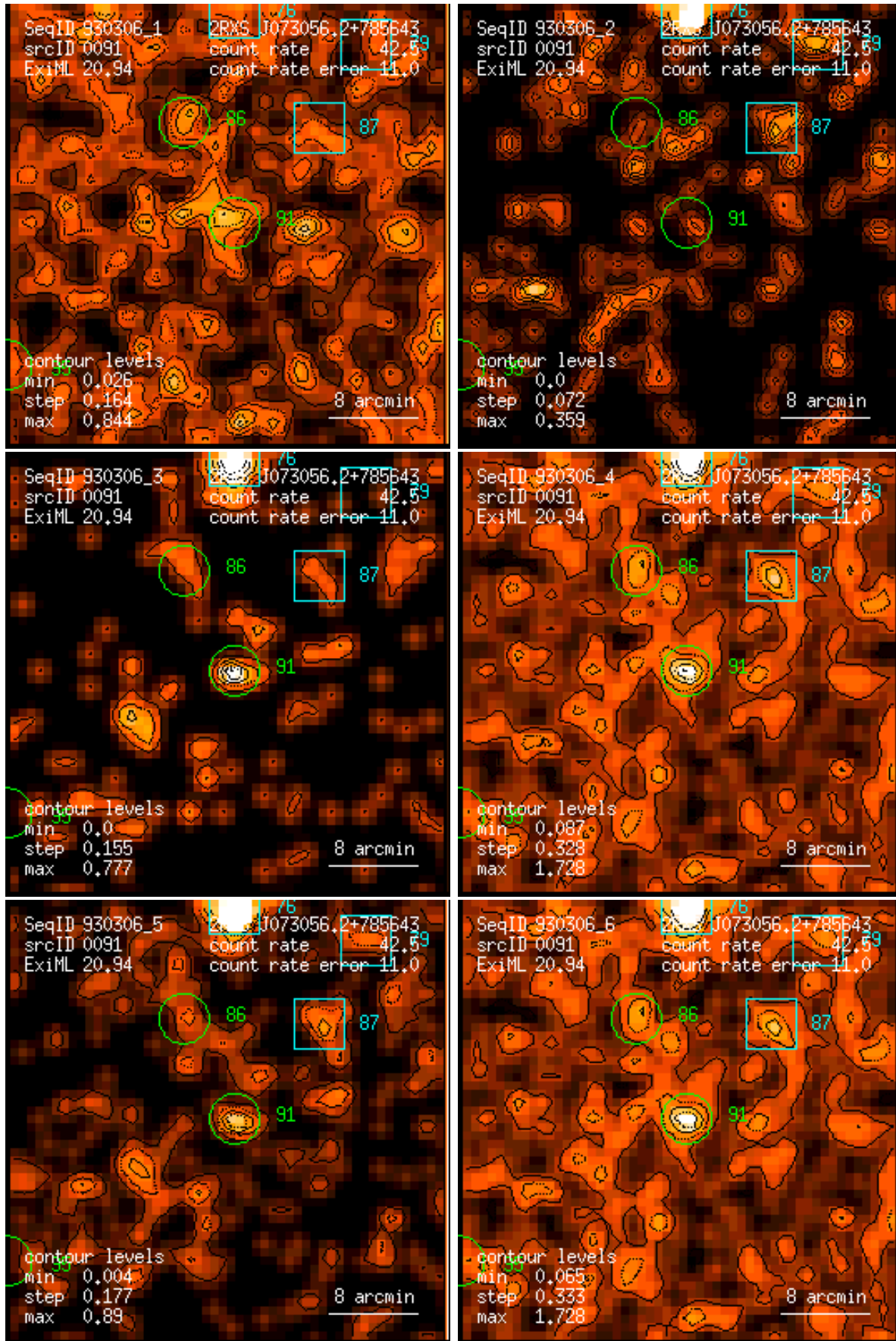
Figure 91: RASS 930306: detection 0091: band rate images, Gaussian filter: (1) PSPC channels 11 – 41, (2) 52 – 90, (3) 91 – 201, (4) 11 – 235, (5) 52 – 201, (6) 11 – 201. Broad band rates in counts/ks. Band rate contour levels in counts/ks/arcmin 2 .
