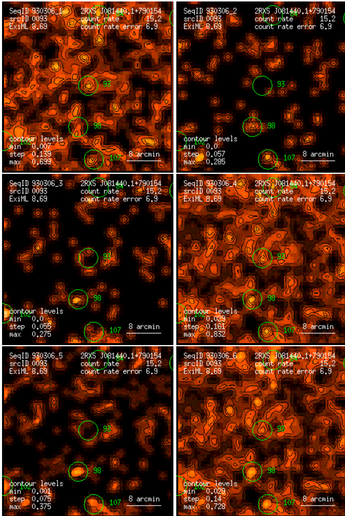
Figure 93: RASS 930306: detection 0093: band rate images, Gaussian filter: (1) PSPC channels 11 – 41, (2) 52 – 90, (3) 91 – 201, (4) 11 – 235, (5) 52 – 201, (6) 11 – 201. Broad band rates in counts/ks. Band rate contour levels in counts/ks/arcmin 2 .
