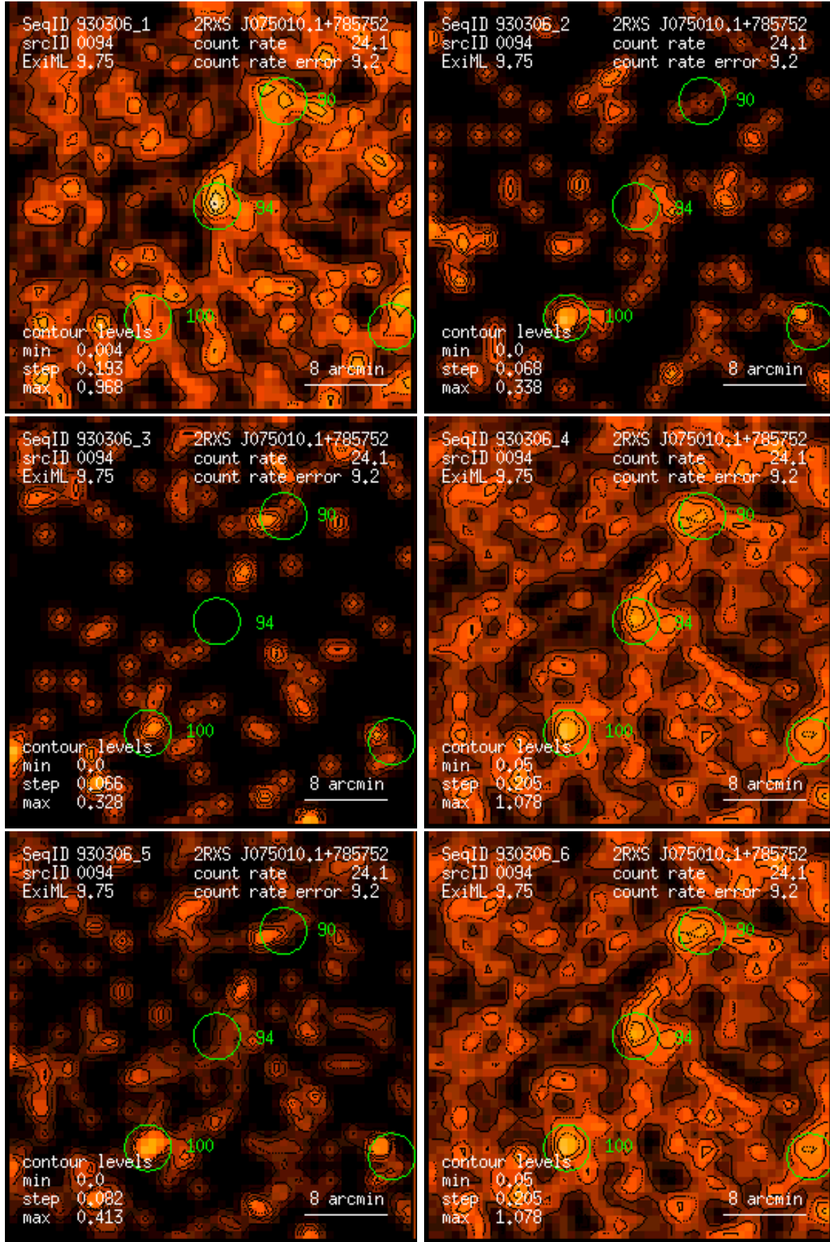
Figure 94: RASS 930306: detection 0094: band rate images, Gaussian filter: (1) PSPC channels 11 – 41, (2) 52 – 90, (3) 91 – 201, (4) 11 – 235, (5) 52 – 201, (6) 11 – 201. Broad band rates in counts/ks. Band rate contour levels in counts/ks/arcmin 2 .
