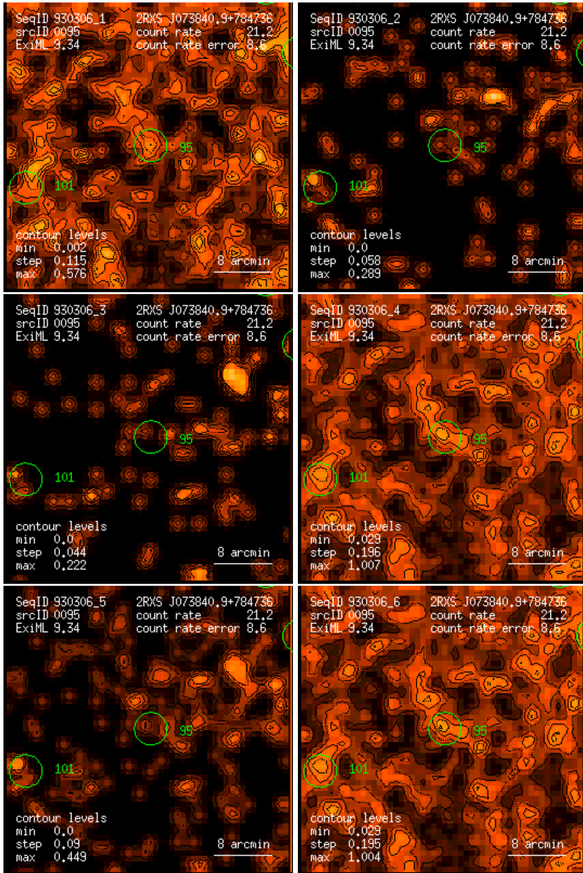
Figure 95: RASS 930306: detection 0095: band rate images, Gaussian filter: (1) PSPC channels 11 – 41, (2) 52 – 90, (3) 91 – 201, (4) 11 – 235, (5) 52 – 201, (6) 11 – 201. Broad band rates in counts/ks. Band rate contour levels in counts/ks/arcmin 2 .
