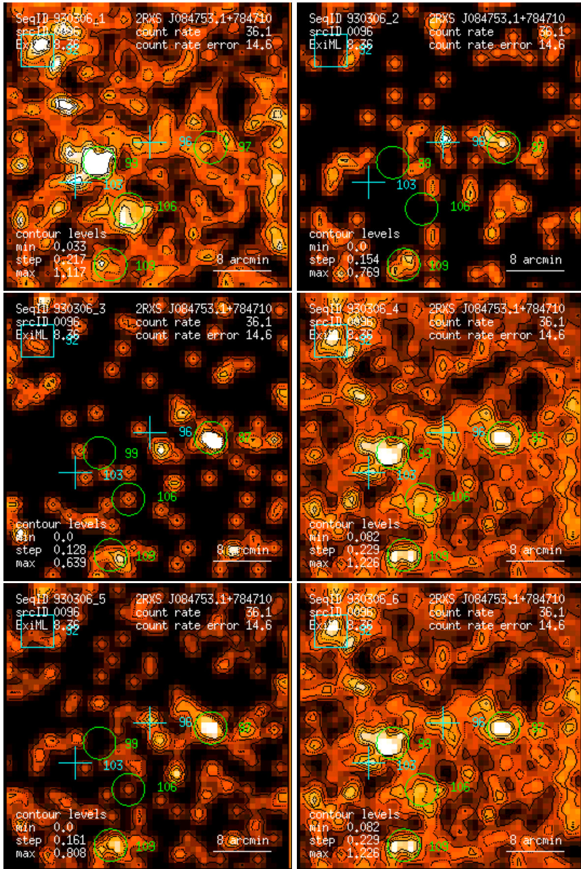
Figure 96: RASS 930306: detection 0096: band rate images, Gaussian filter: (1) PSPC channels 11 – 41, (2) 52 – 90, (3) 91 – 201, (4) 11 – 235, (5) 52 – 201, (6) 11 – 201. Broad band rates in counts/ks. Band rate contour levels in counts/ks/arcmin 2 .
