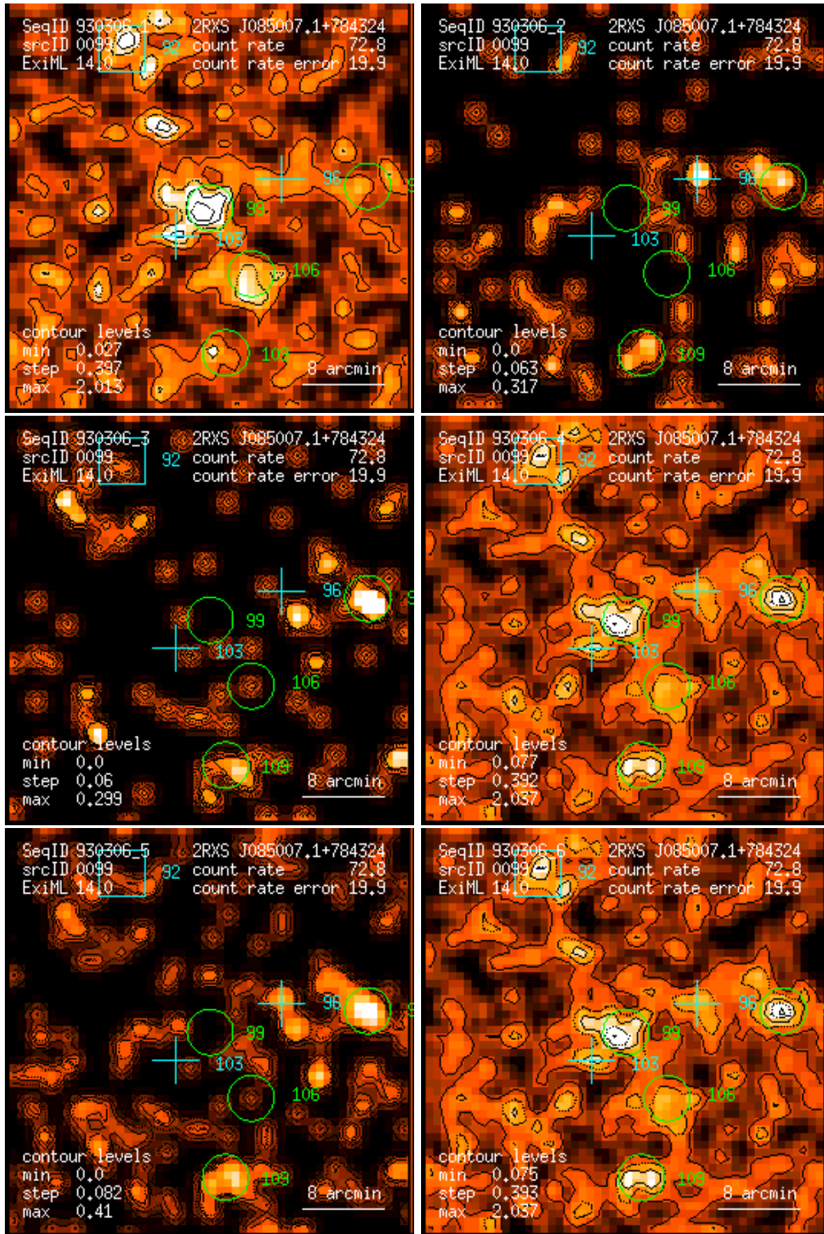
Figure 99: RASS 930306: detection 0099: band rate images, Gaussian filter: (1) PSPC channels 11 – 41, (2) 52 – 90, (3) 91 – 201, (4) 11 – 235, (5) 52 – 201, (6) 11 – 201. Broad band rates in counts/ks. Band rate contour levels in counts/ks/arcmin 2 .
