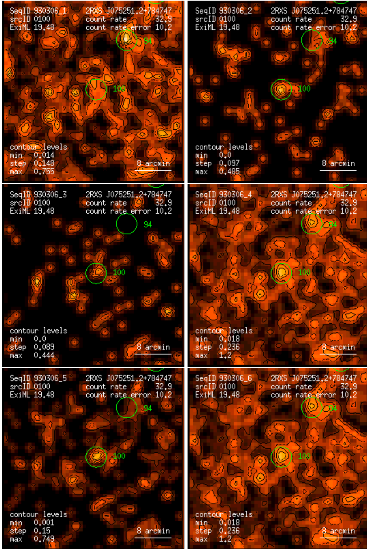
Figure 100: RASS 930306: detection 0100: band rate images, Gaussian filter: (1) PSPC channels 11 – 41, (2) 52 – 90, (3) 91 – 201, (4) 11 – 235, (5) 52 – 201, (6) 11 – 201. Broad band rates in counts/ks. Band rate contour levels in counts/ks/arcmin 2 .
