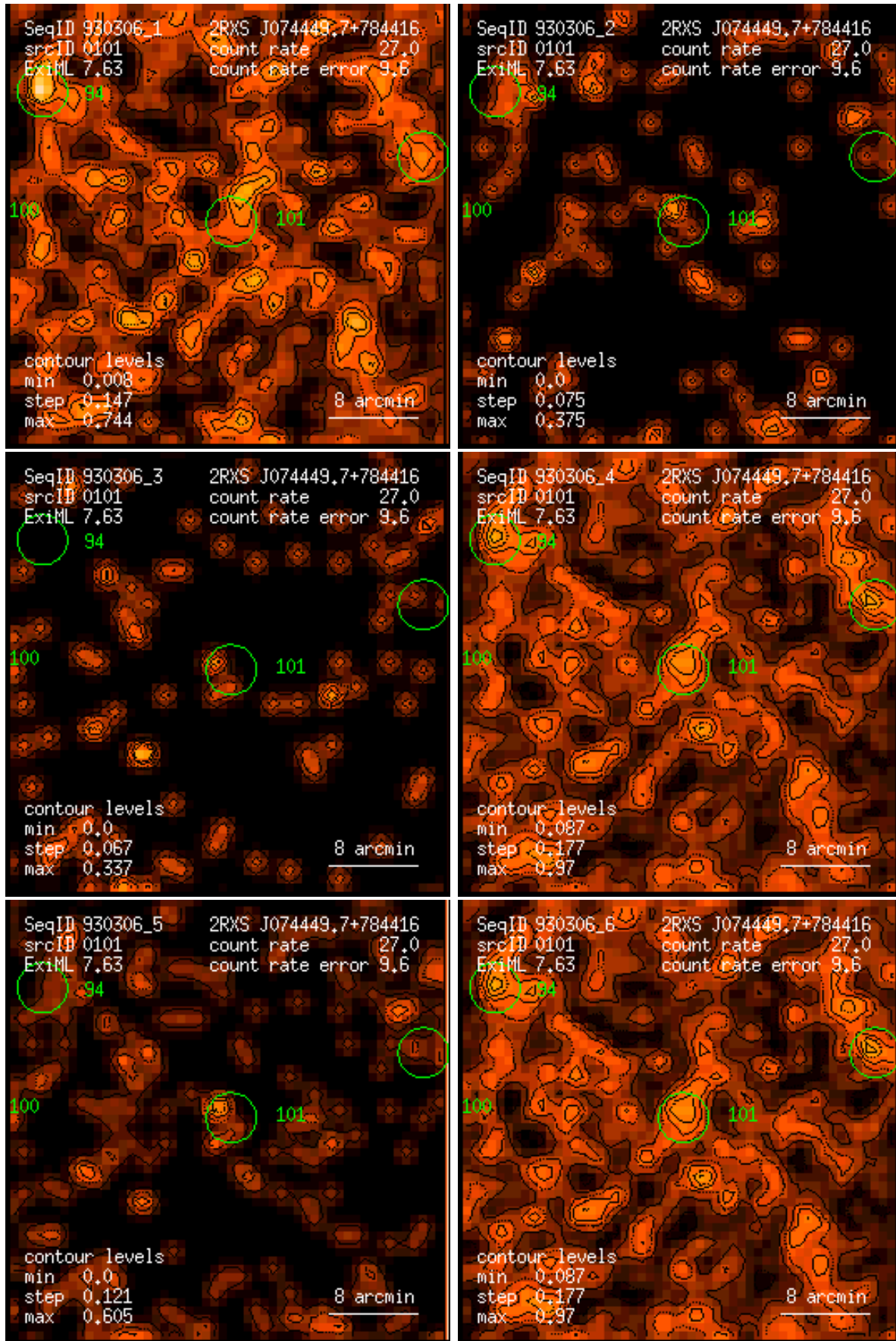
Figure 101: RASS 930306: detection 0101: band rate images, Gaussian filter: (1) PSPC channels 11 – 41, (2) 52 – 90, (3) 91 – 201, (4) 11 – 235, (5) 52 – 201, (6) 11 – 201. Broad band rates in counts/ks. Band rate contour levels in counts/ks/arcmin 2 .
