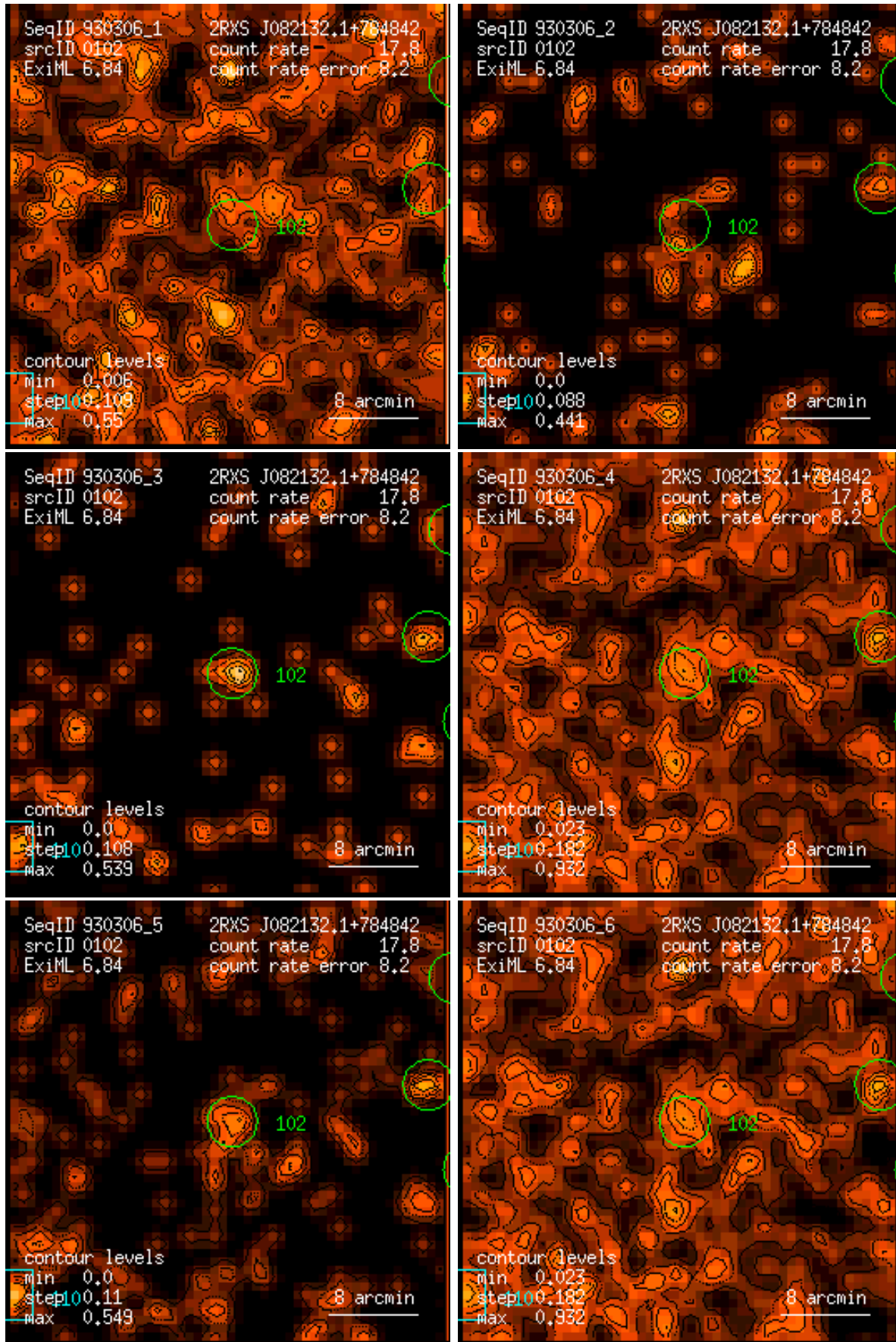
Figure 102: RASS 930306: detection 0102: band rate images, Gaussian filter: (1) PSPC channels 11 – 41, (2) 52 – 90, (3) 91 – 201, (4) 11 – 235, (5) 52 – 201, (6) 11 – 201. Broad band rates in counts/ks. Band rate contour levels in counts/ks/arcmin 2 .
