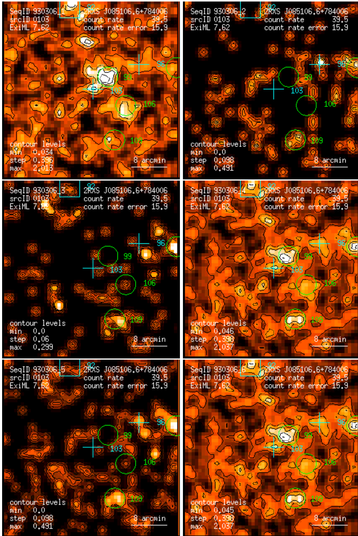
Figure 103: RASS 930306: detection 0103: band rate images, Gaussian filter: (1) PSPC channels 11 – 41, (2) 52 – 90, (3) 91 – 201, (4) 11 – 235, (5) 52 – 201, (6) 11 – 201. Broad band rates in counts/ks. Band rate contour levels in counts/ks/arcmin 2 .
