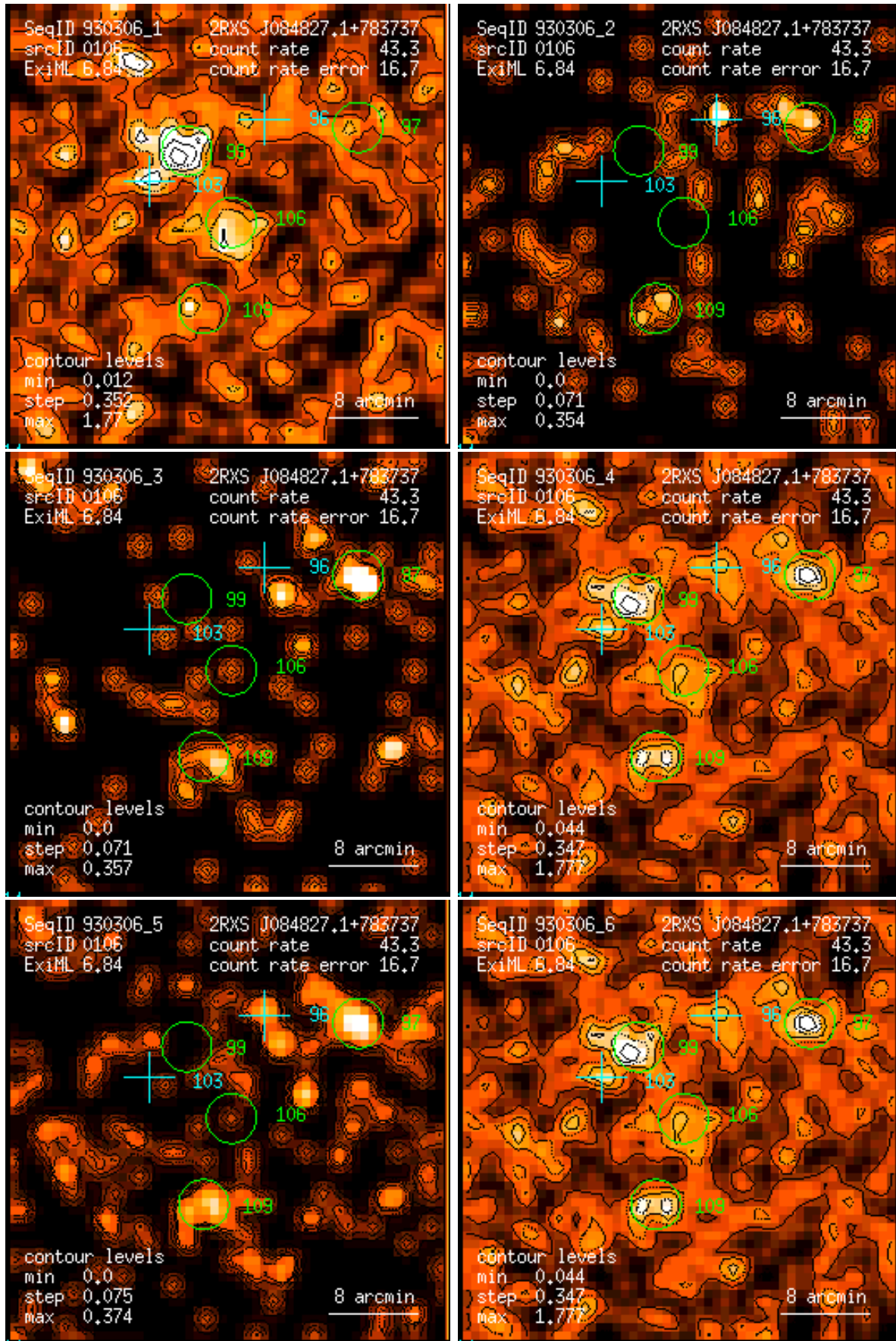
Figure 106: RASS 930306: detection 0106: band rate images, Gaussian filter: (1) PSPC channels 11 – 41, (2) 52 – 90, (3) 91 – 201, (4) 11 – 235, (5) 52 – 201, (6) 11 – 201. Broad band rates in counts/ks. Band rate contour levels in counts/ks/arcmin 2 .
