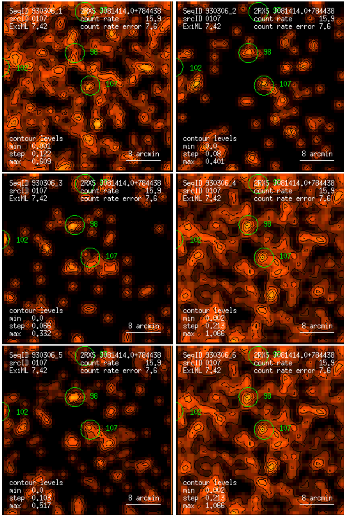
Figure 107: RASS 930306: detection 0107: band rate images, Gaussian filter: (1) PSPC channels 11 – 41, (2) 52 – 90, (3) 91 – 201, (4) 11 – 235, (5) 52 – 201, (6) 11 – 201. Broad band rates in counts/ks. Band rate contour levels in counts/ks/arcmin 2 .
