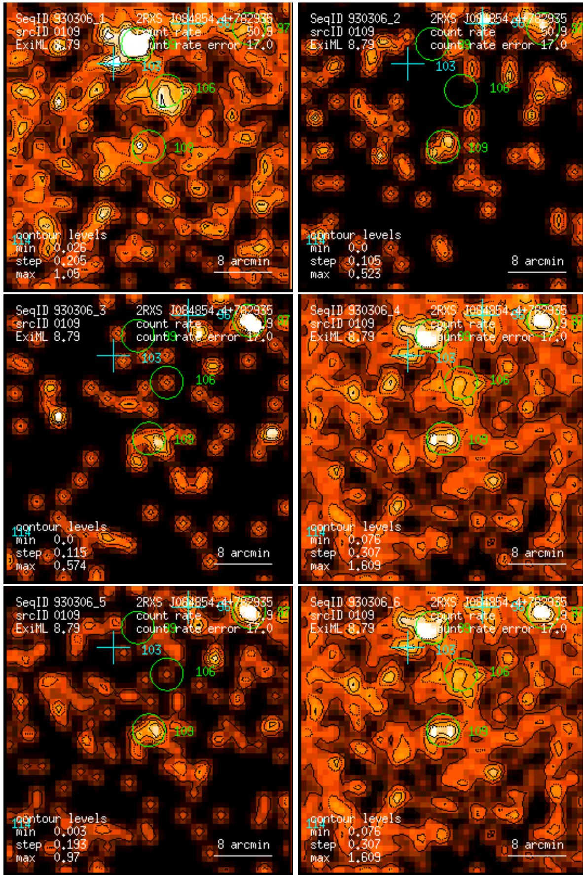
Figure 109: RASS 930306: detection 0109: band rate images, Gaussian filter: (1) PSPC channels 11 – 41, (2) 52 – 90, (3) 91 – 201, (4) 11 – 235, (5) 52 – 201, (6) 11 – 201. Broad band rates in counts/ks. Band rate contour levels in counts/ks/arcmin 2 .
