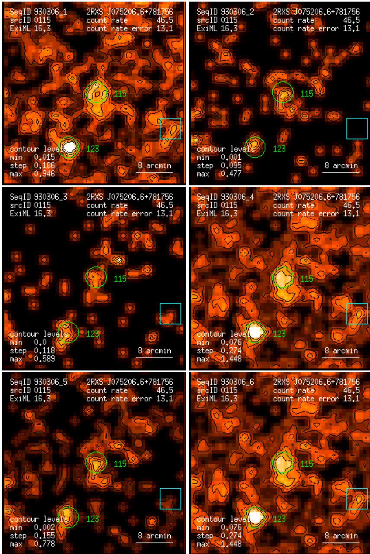
Figure 115: RASS 930306: detection 0115: band rate images, Gaussian filter: (1) PSPC channels 11 – 41, (2) 52 – 90, (3) 91 – 201, (4) 11 – 235, (5) 52 – 201, (6) 11 – 201. Broad band rates in counts/ks. Band rate contour levels in counts/ks/arcmin 2 .
