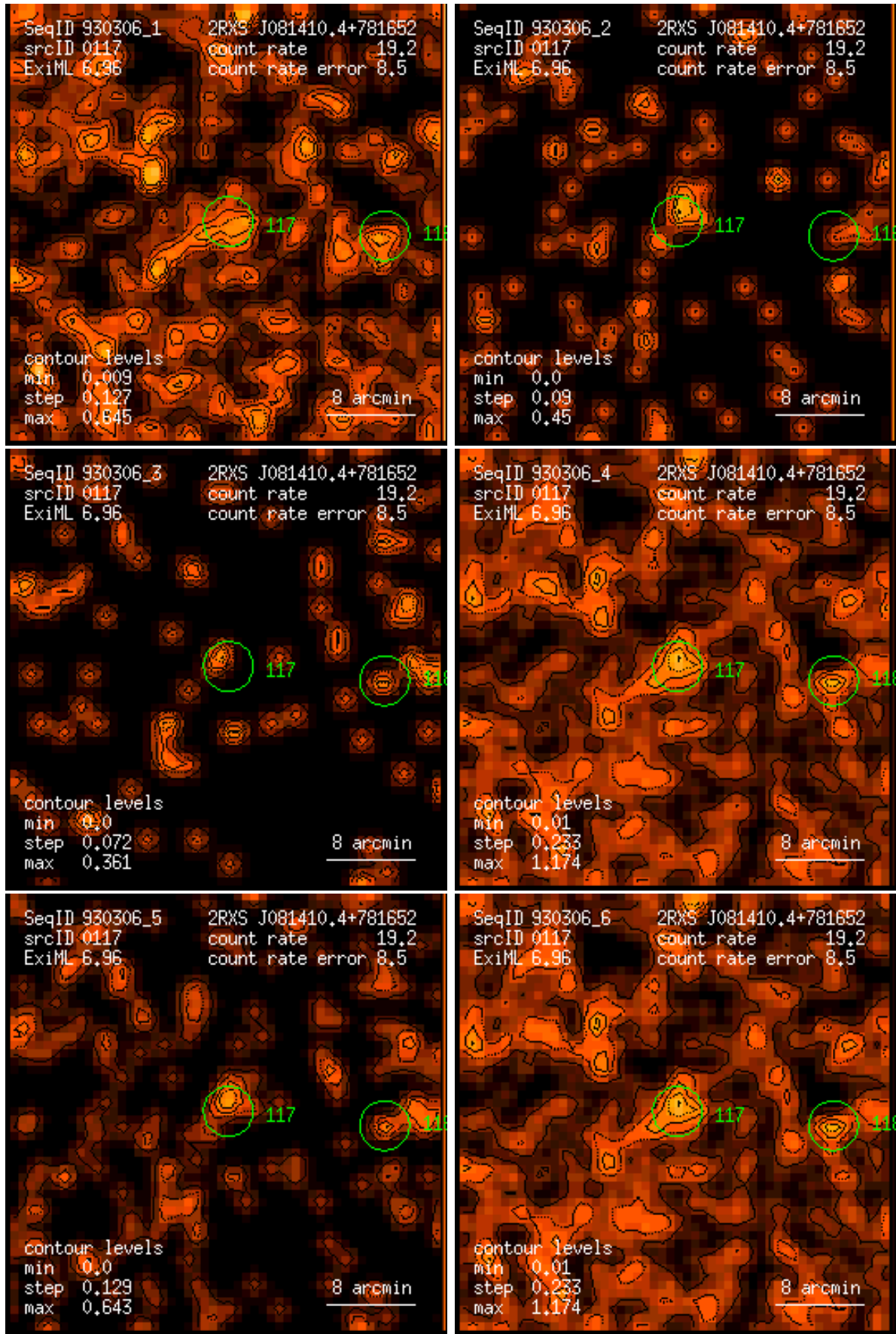
Figure 117: RASS 930306: detection 0117: band rate images, Gaussian filter: (1) PSPC channels 11 – 41, (2) 52 – 90, (3) 91 – 201, (4) 11 – 235, (5) 52 – 201, (6) 11 – 201. Broad band rates in counts/ks. Band rate contour levels in counts/ks/arcmin 2 .
