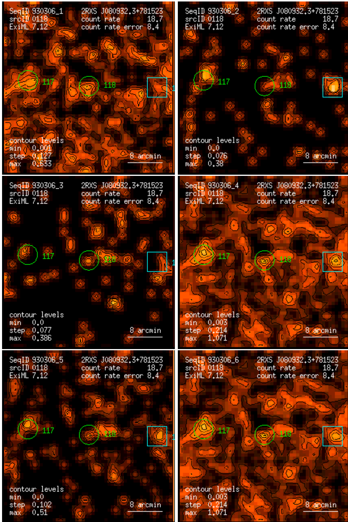
Figure 118: RASS 930306: detection 0118: band rate images, Gaussian filter: (1) PSPC channels 11 – 41, (2) 52 – 90, (3) 91 – 201, (4) 11 – 235, (5) 52 – 201, (6) 11 – 201. Broad band rates in counts/ks. Band rate contour levels in counts/ks/arcmin 2 .
